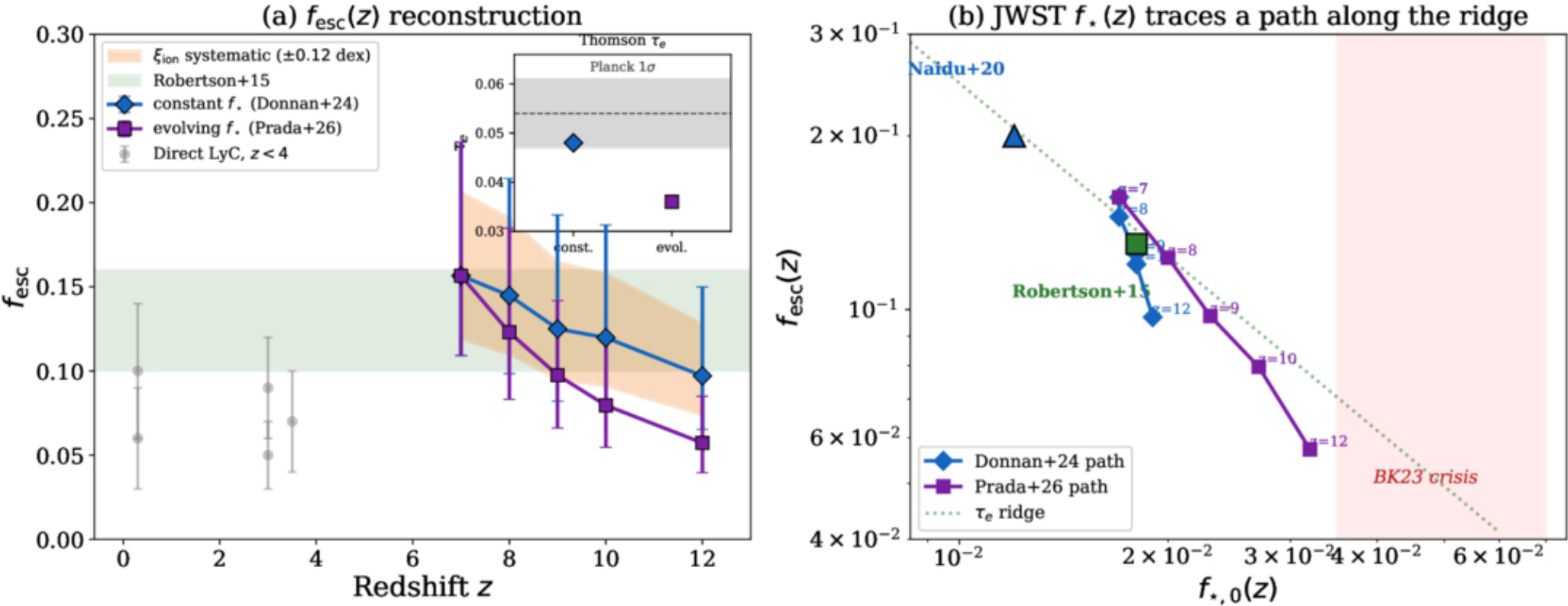
Figure 4. from Zihan Wang and Huanyuan Shan 2026 Astrophys. J. Lett. 1006 doi:10.3847/2041-8213/ae88f1 https://dx.doi.org/10.3847/2041-8213/ae88f1 © 2026. The Author(s). Published by the American Astronomical Society.
