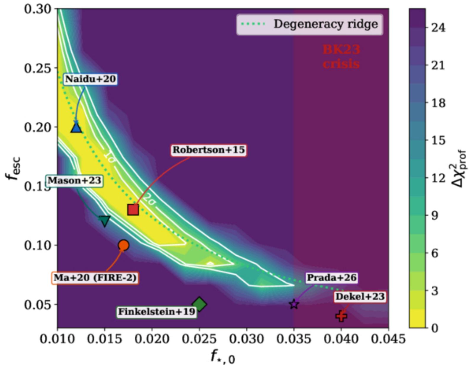
Figure 2. from Zihan Wang and Huanyuan Shan 2026 Astrophys. J. Lett. 1006 doi:10.3847/2041-8213/ae88f1 https://dx.doi.org/10.3847/2041-8213/ae88f1 © 2026. The Author(s). Published by the American Astronomical Society.
