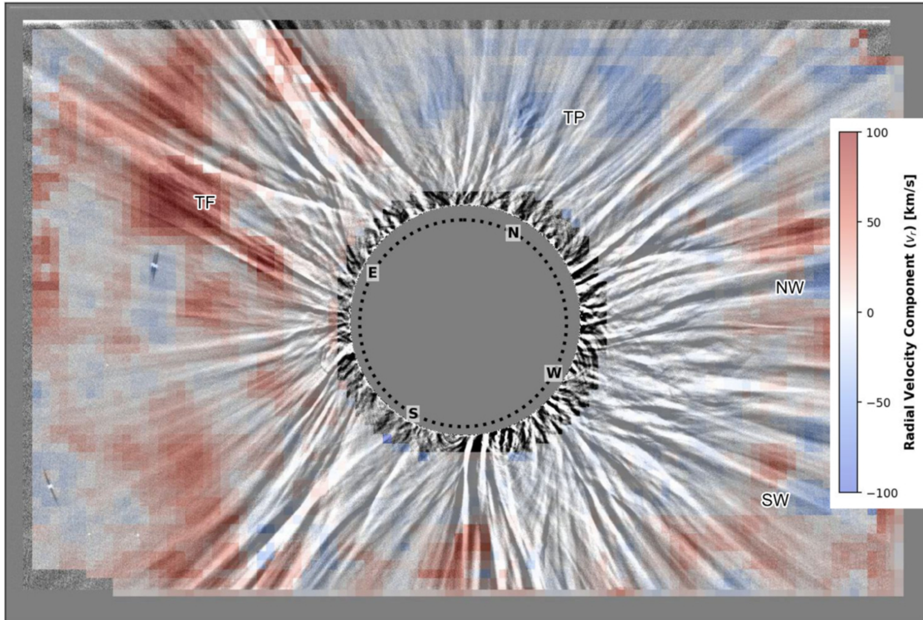
Figure 4. from Matthew J Penn et al 2026 Astrophys. J. Lett. 1006 doi:10.3847/2041-8213/ae8797 https://dx.doi.org/10.3847/2041-8213/ae8797 © 2026. The Author(s). Published by the American Astronomical Society.
