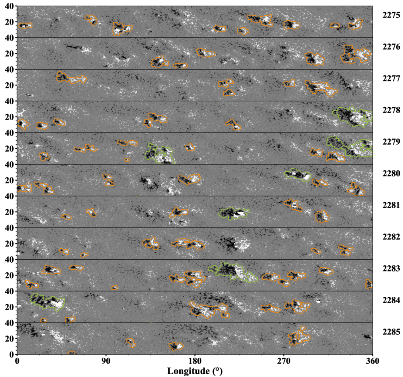
Figure 4. from Zi-Fan Wang et al 2026 Astrophys. J. Lett. 1006 doi:10.3847/2041-8213/ae8765 https://dx.doi.org/10.3847/2041-8213/ae8765 © 2026. The Author(s). Published by the American Astronomical Society.
