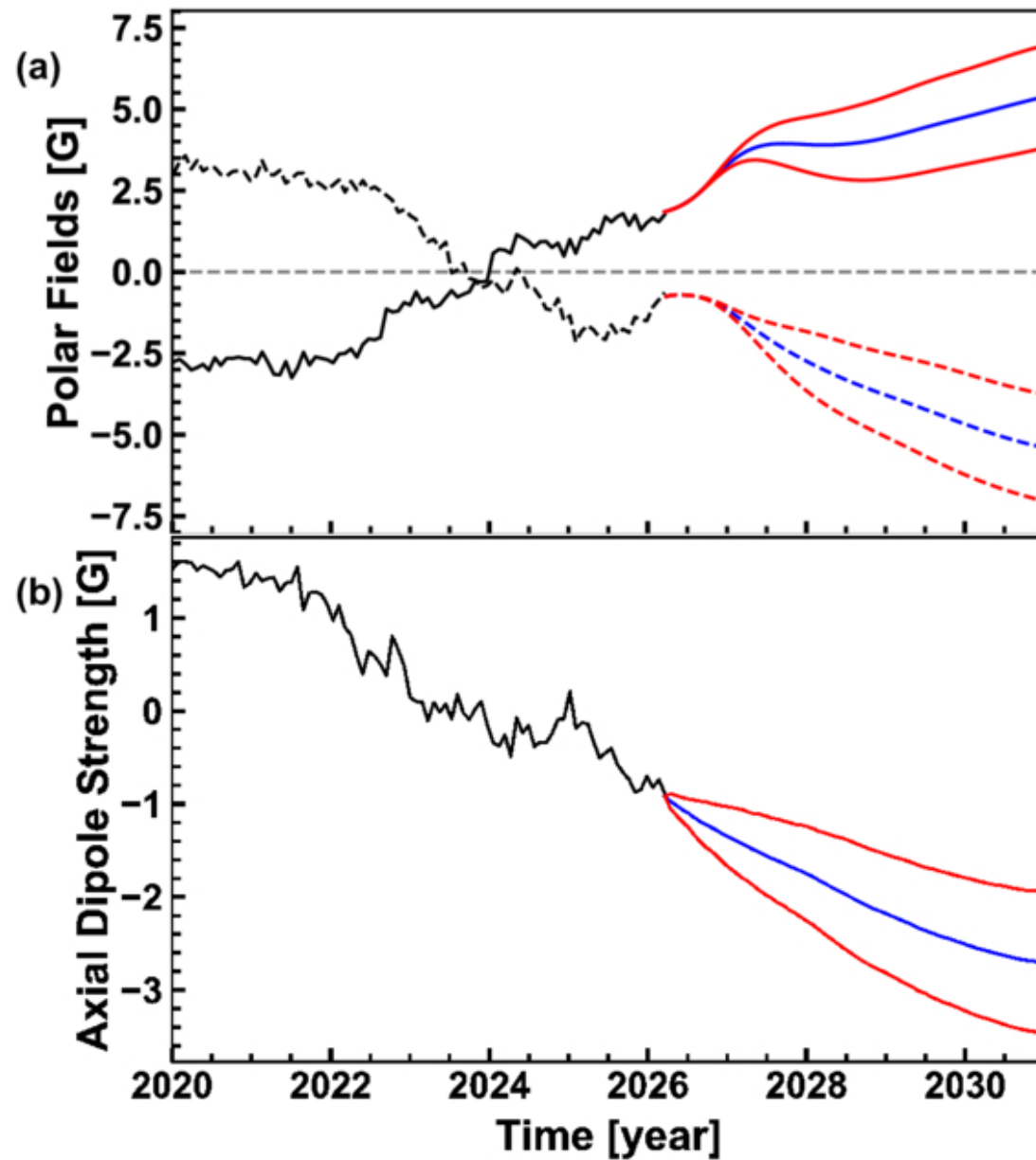
Figure 3. from Zi-Fan Wang et al 2026 Astrophys. J. Lett. 1006 doi:10.3847/2041-8213/ae8765 https://dx.doi.org/10.3847/2041-8213/ae8765 © 2026. The Author(s). Published by the American Astronomical Society.
