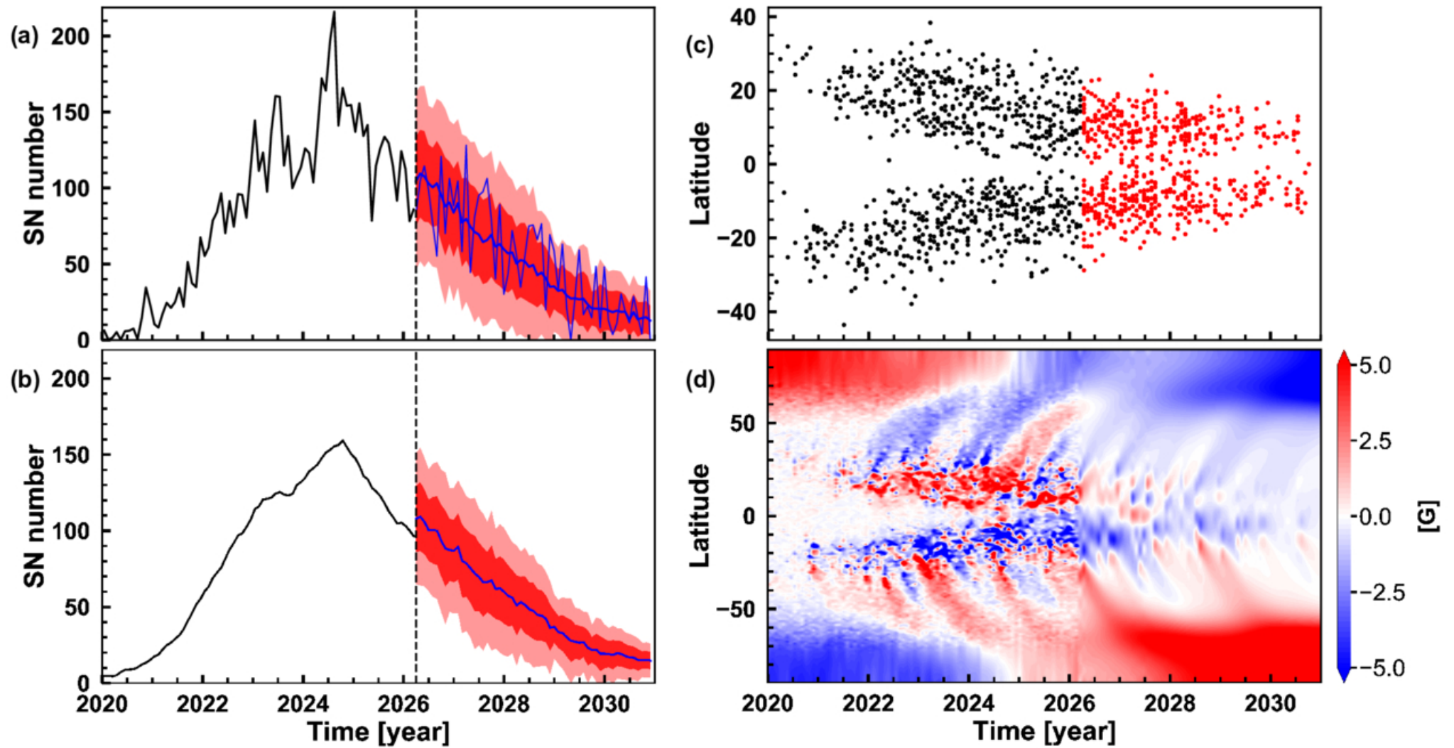
Figure 2. from Zi-Fan Wang et al 2026 Astrophys. J. Lett. 1006 doi:10.3847/2041-8213/ae8765 https://dx.doi.org/10.3847/2041-8213/ae8765 © 2026. The Author(s). Published by the American Astronomical Society.
