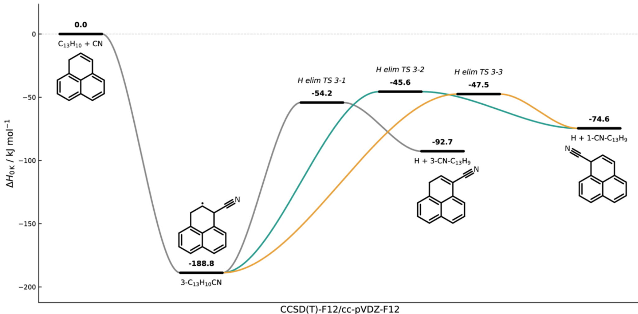
Figure C2. from Gabi Wenzel et al 2026 Astrophys. J. Lett. 1006 doi:10.3847/2041-8213/ae8757 https://dx.doi.org/10.3847/2041-8213/ae8757 © 2026. The Author(s). Published by the American Astronomical Society.
