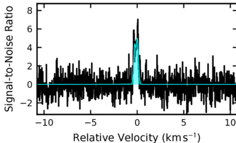
Figure A1. from Gabi Wenzel et al 2026 Astrophys. J. Lett. 1006 doi:10.3847/2041-8213/ae8757 https://dx.doi.org/10.3847/2041-8213/ae8757 © 2026. The Author(s). Published by the American Astronomical Society.
