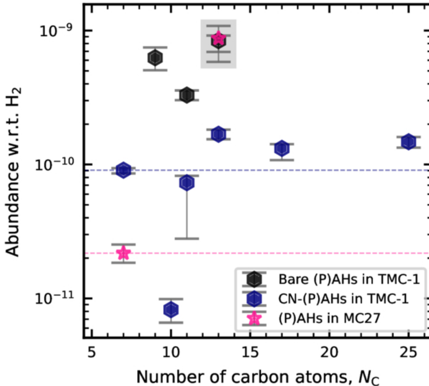
Figure 2. from Gabi Wenzel et al 2026 Astrophys. J. Lett. 1006 doi:10.3847/2041-8213/ae8757 https://dx.doi.org/10.3847/2041-8213/ae8757 © 2026. The Author(s). Published by the American Astronomical Society.
