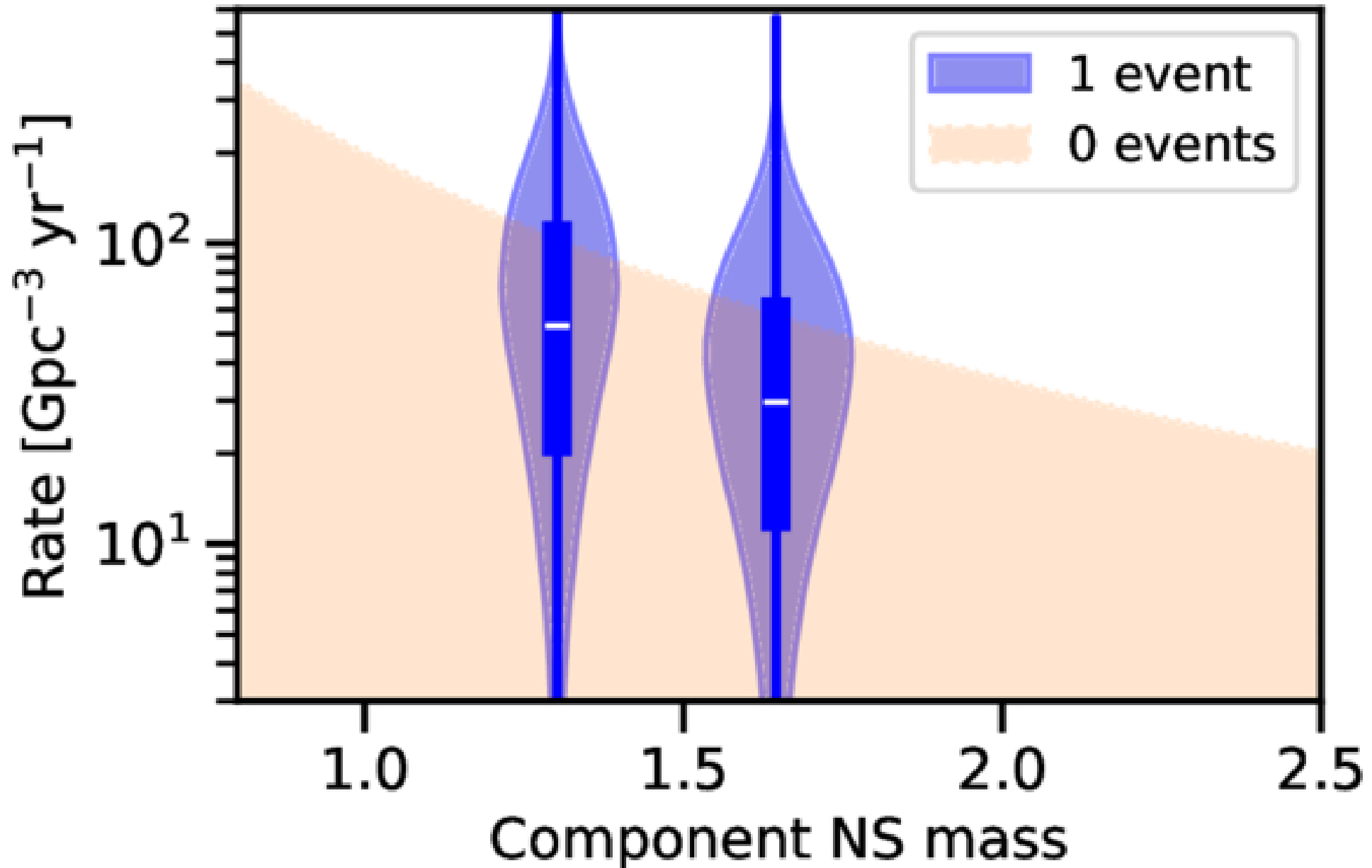
Figure 3. from Maya Fishbach et al 2026 Astrophys. J. Lett. 1006 doi:10.3847/2041-8213/ae8756 https://dx.doi.org/10.3847/2041-8213/ae8756 © 2026. The Author(s). Published by the American Astronomical Society.
