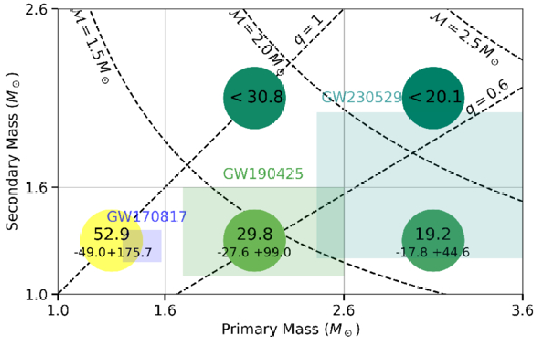
Figure 2. from Maya Fishbach et al 2026 Astrophys. J. Lett. 1006 doi:10.3847/2041-8213/ae8756 https://dx.doi.org/10.3847/2041-8213/ae8756 © 2026. The Author(s). Published by the American Astronomical Society.
