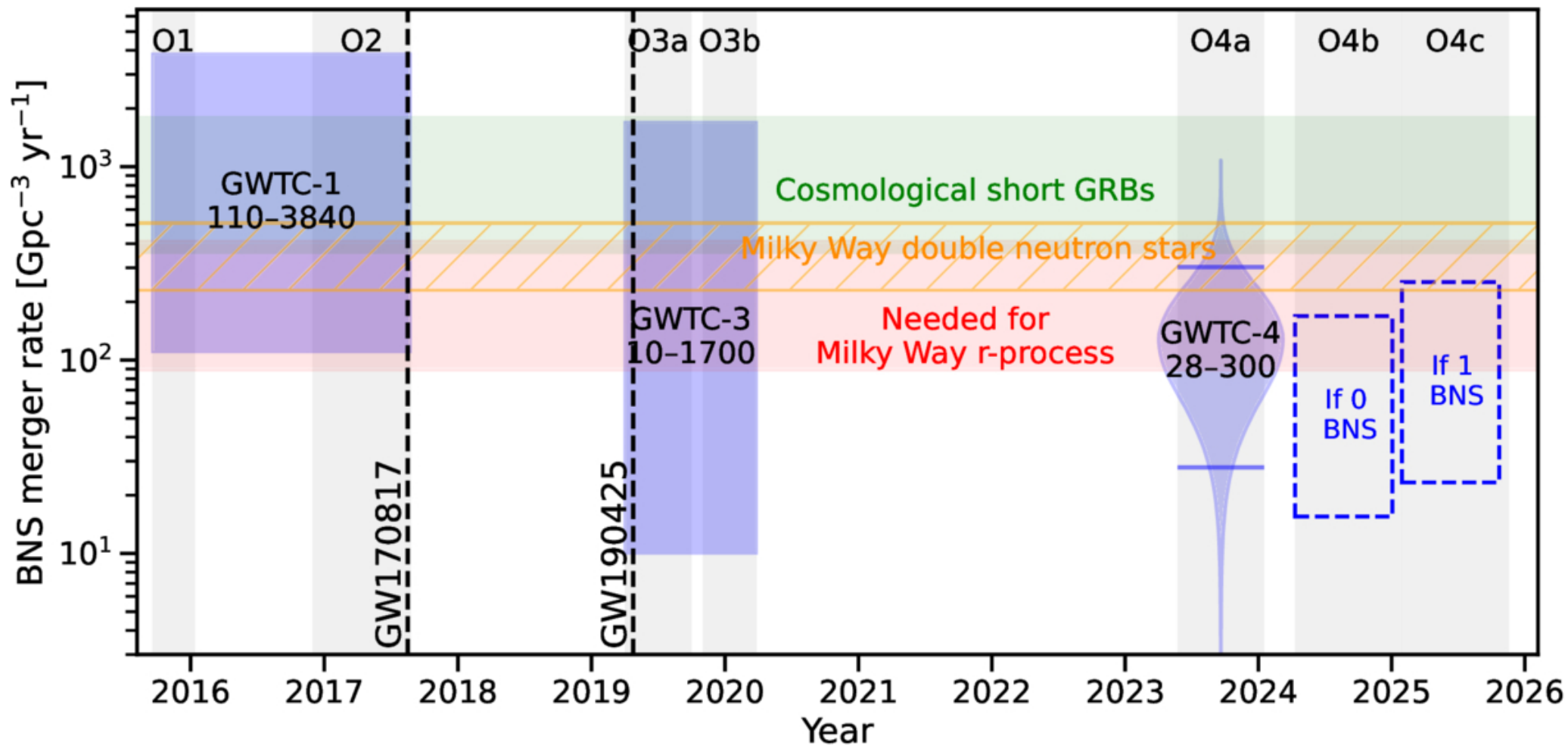
Figure 1. from Maya Fishbach et al 2026 Astrophys. J. Lett. 1006 doi:10.3847/2041-8213/ae8756 https://dx.doi.org/10.3847/2041-8213/ae8756 © 2026. The Author(s). Published by the American Astronomical Society.
