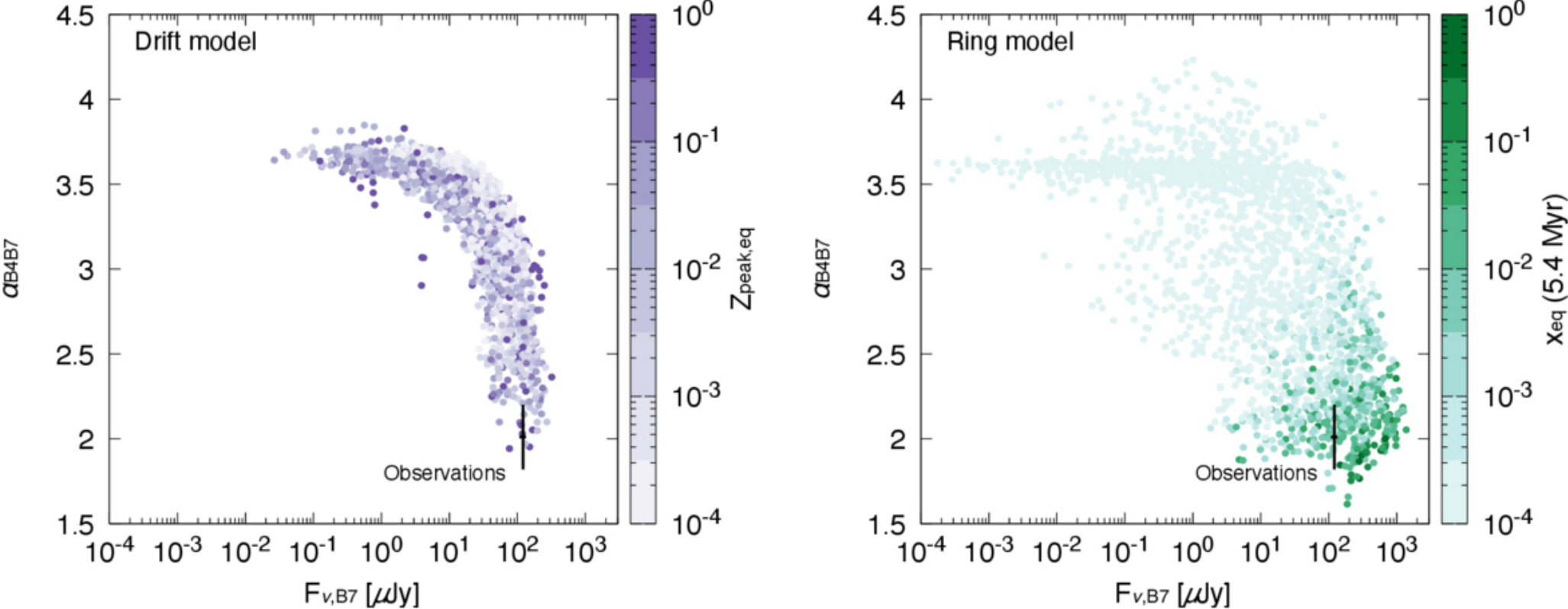
Figure 5. from Yuhito Shibaike et al 2026 Astrophys. J. Lett. 1006 doi:10.3847/2041-8213/ae86f5 https://dx.doi.org/10.3847/2041-8213/ae86f5 © 2026. The Author(s). Published by the American Astronomical Society.
