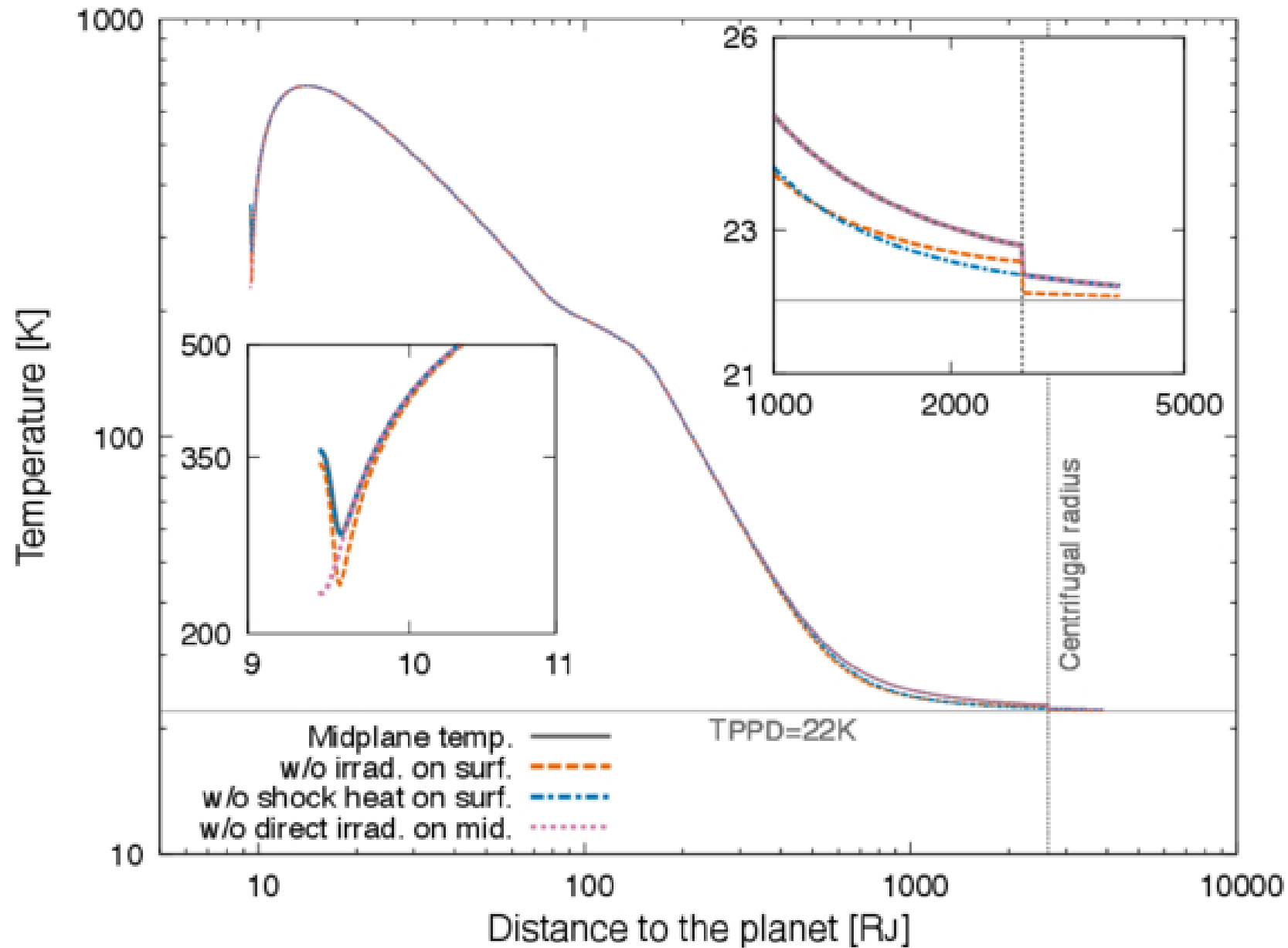
Figure 4. from Yuhito Shibaike et al 2026 Astrophys. J. Lett. 1006 doi:10.3847/2041-8213/ae86f5 https://dx.doi.org/10.3847/2041-8213/ae86f5 © 2026. The Author(s). Published by the American Astronomical Society.
