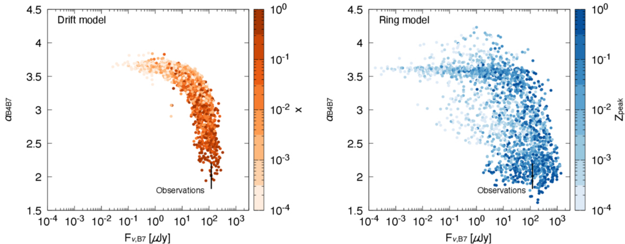
Figure 3. from Yuhito Shibaike et al 2026 Astrophys. J. Lett. 1006 doi:10.3847/2041-8213/ae86f5 https://dx.doi.org/10.3847/2041-8213/ae86f5 © 2026. The Author(s). Published by the American Astronomical Society.
