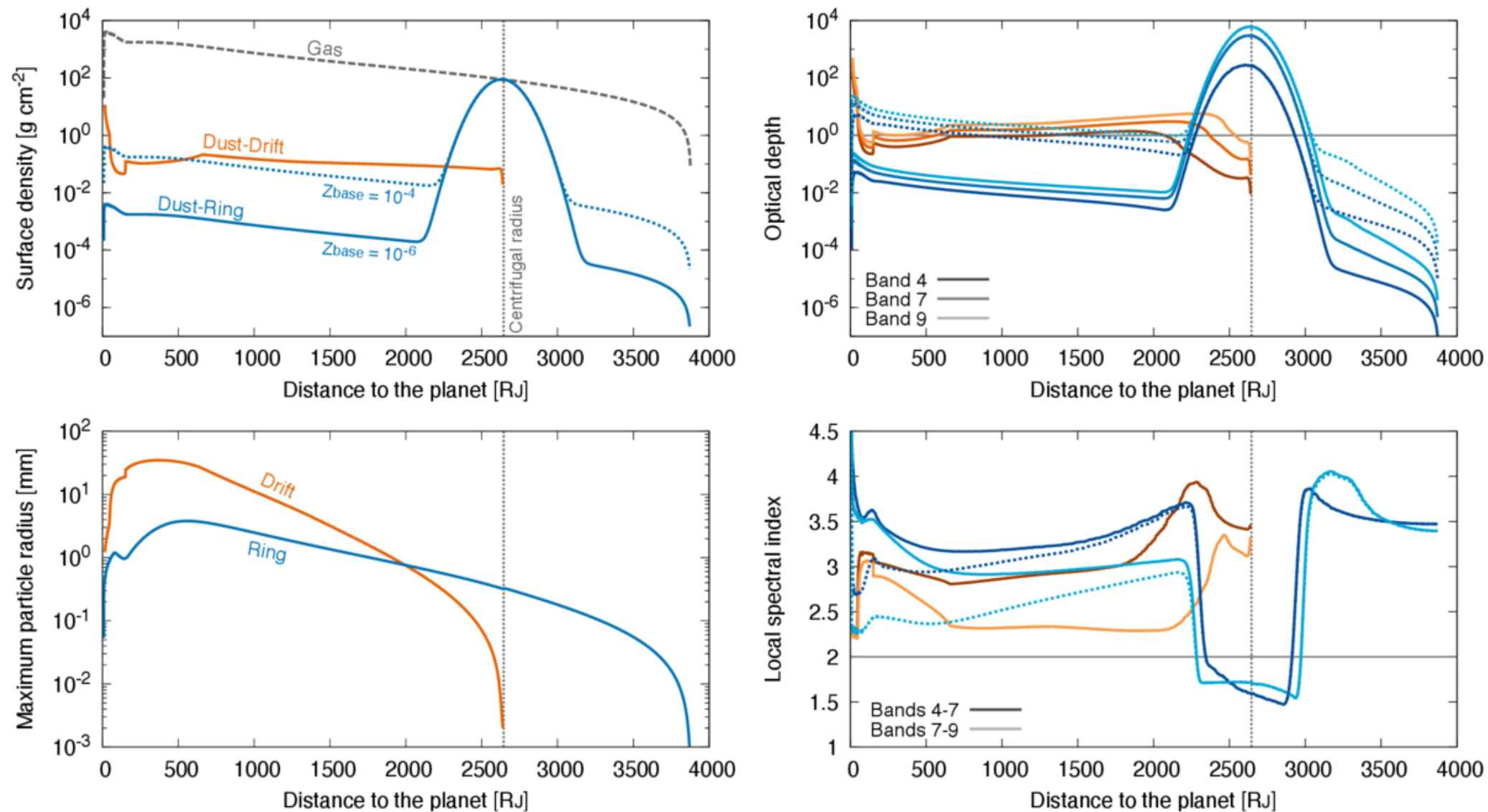
Figure 2. from Yuhito Shibaike et al 2026 Astrophys. J. Lett. 1006 doi:10.3847/2041-8213/ae86f5 https://dx.doi.org/10.3847/2041-8213/ae86f5 © 2026. The Author(s). Published by the American Astronomical Society.
