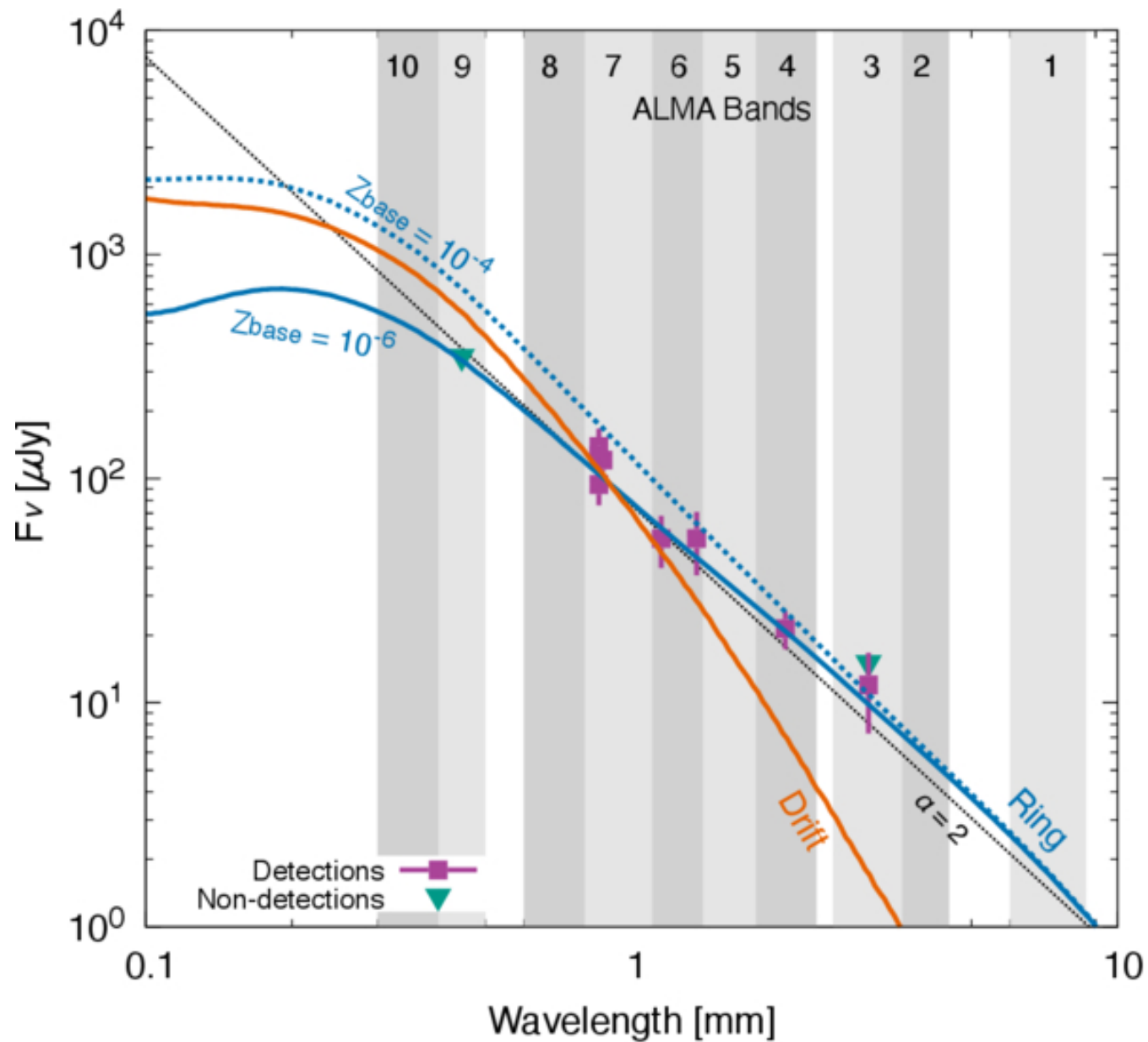
Figure 1. from Yuhito Shibaike et al 2026 Astrophys. J. Lett. 1006 doi:10.3847/2041-8213/ae86f5 https://dx.doi.org/10.3847/2041-8213/ae86f5 © 2026. The Author(s). Published by the American Astronomical Society.
