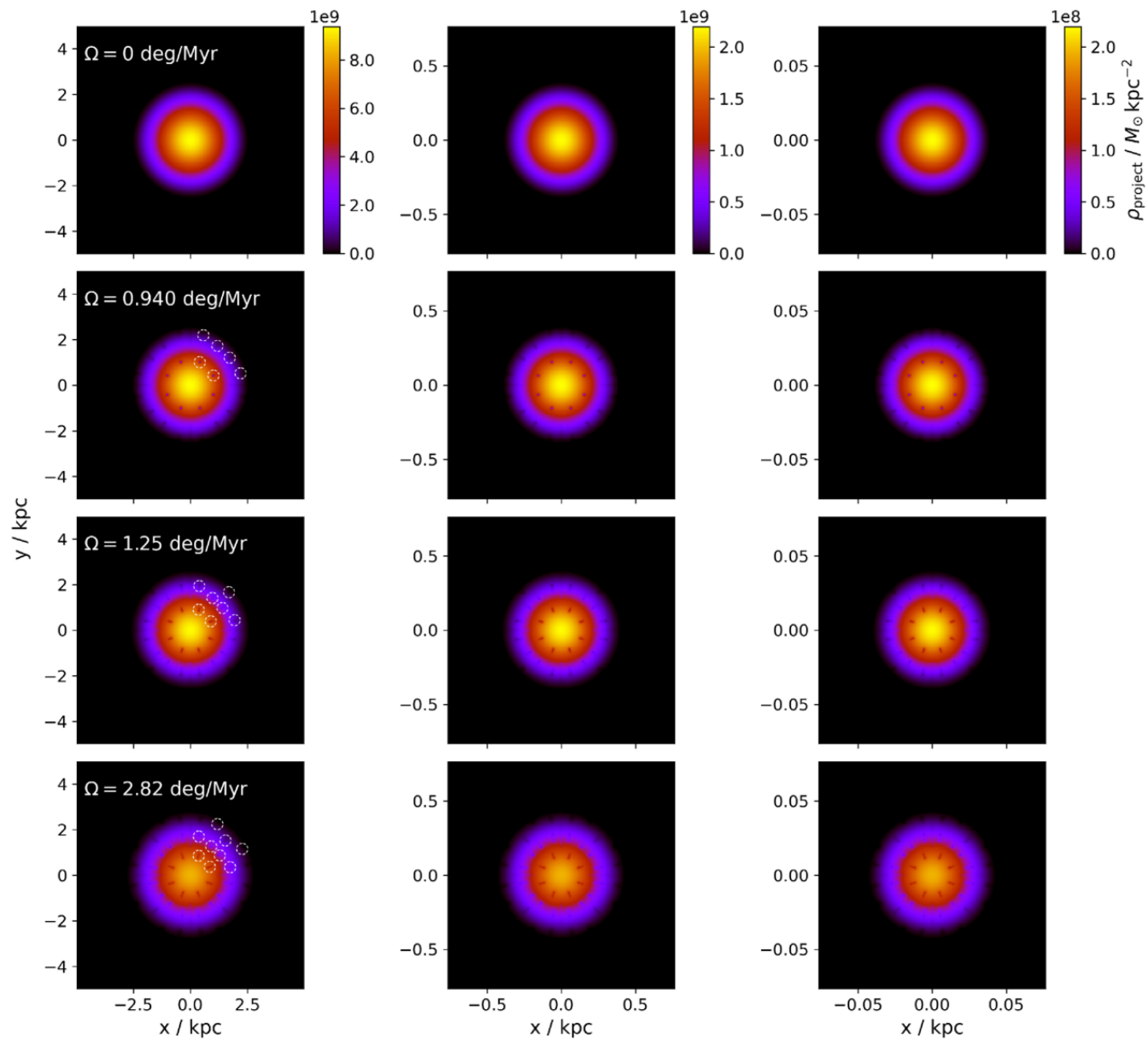
Figure 1. from Rongzi Zhou et al 2026 Astrophys. J. Lett. 1006 doi:10.3847/2041-8213/ae86f1 https://dx.doi.org/10.3847/2041-8213/ae86f1 © 2026. The Author(s). Published by the American Astronomical Society.
