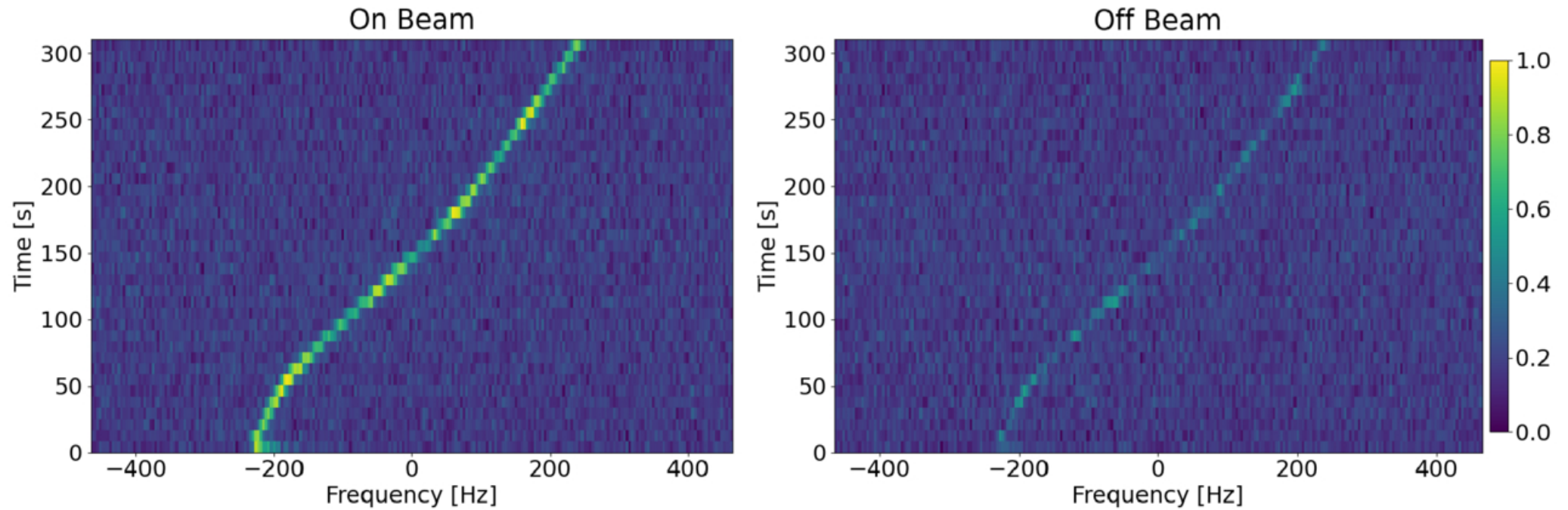
Figure 2. from Chenoa D. Tremblay et al 2026 Astrophys. J. Lett. 1006 doi:10.3847/2041-8213/ae86f0 https://dx.doi.org/10.3847/2041-8213/ae86f0 © 2026. The Author(s). Published by the American Astronomical Society.
