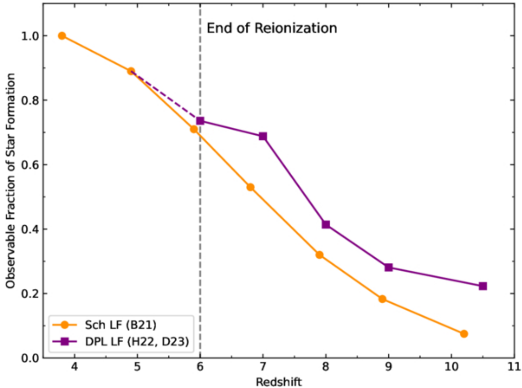
Figure 5. from Jing-Meng Hao et al 2026 Astrophys. J. Lett. 1006 doi:10.3847/2041-8213/ae86ef https://dx.doi.org/10.3847/2041-8213/ae86ef © 2026. The Author(s). Published by the American Astronomical Society.
