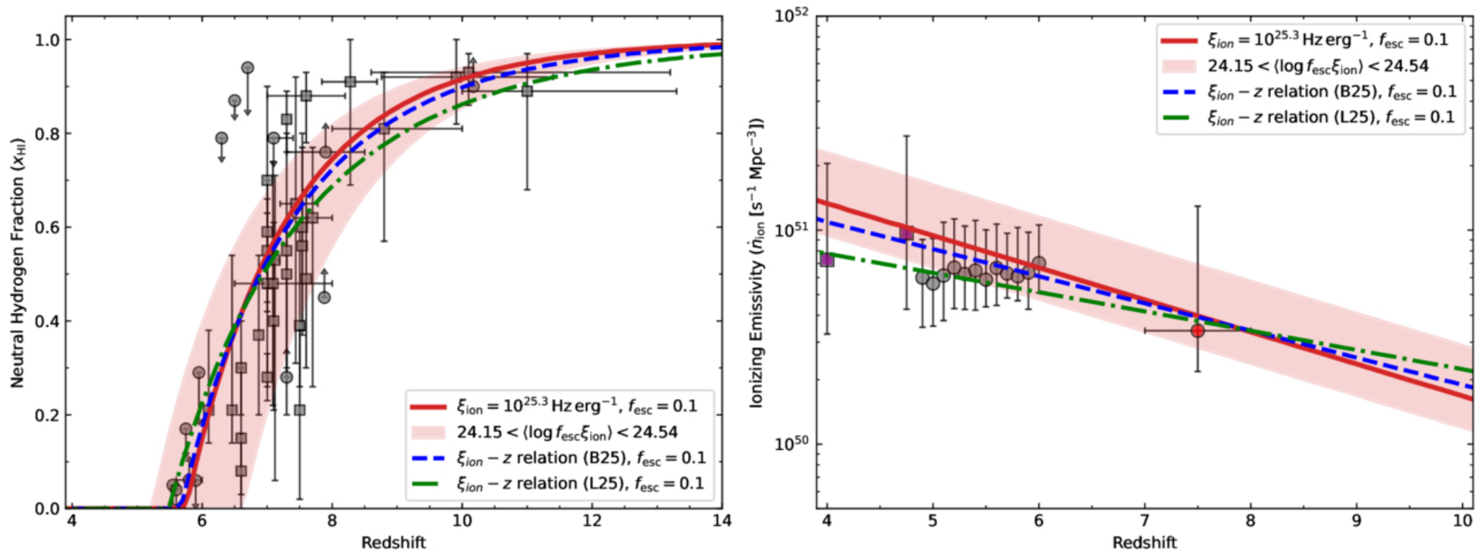
Figure 3. from Jing-Meng Hao et al 2026 Astrophys. J. Lett. 1006 doi:10.3847/2041-8213/ae86ef https://dx.doi.org/10.3847/2041-8213/ae86ef © 2026. The Author(s). Published by the American Astronomical Society.
