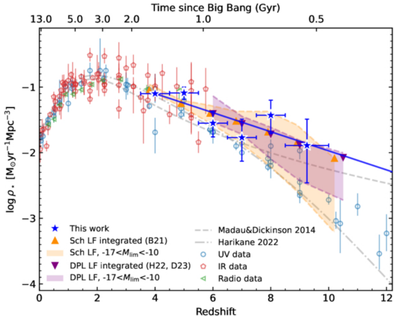
Figure 2. from Jing-Meng Hao et al 2026 Astrophys. J. Lett. 1006 doi:10.3847/2041-8213/ae86ef https://dx.doi.org/10.3847/2041-8213/ae86ef © 2026. The Author(s). Published by the American Astronomical Society.
