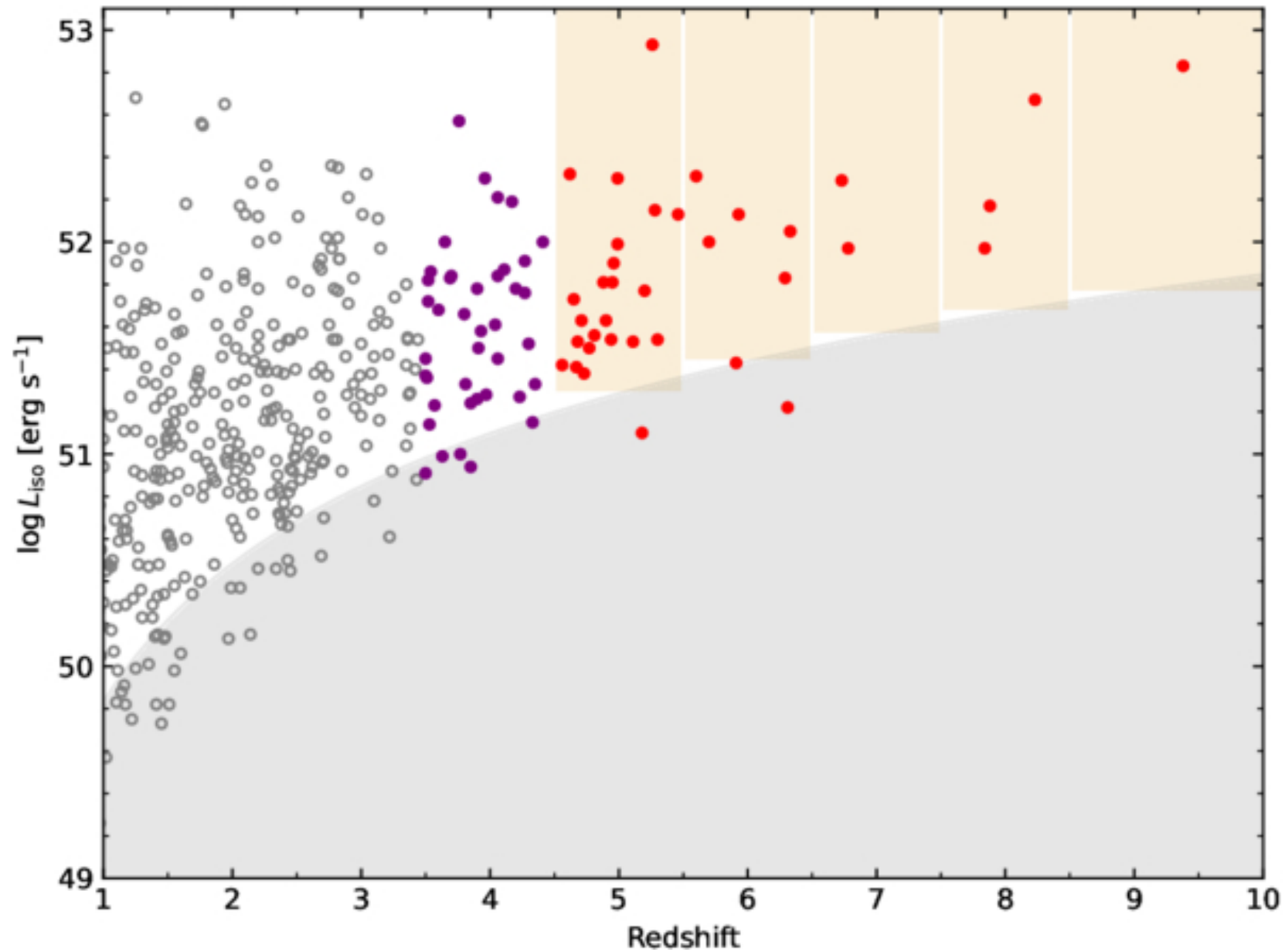
Figure 1. from Jing-Meng Hao et al 2026 Astrophys. J. Lett. 1006 doi:10.3847/2041-8213/ae86ef https://dx.doi.org/10.3847/2041-8213/ae86ef © 2026. The Author(s). Published by the American Astronomical Society.
