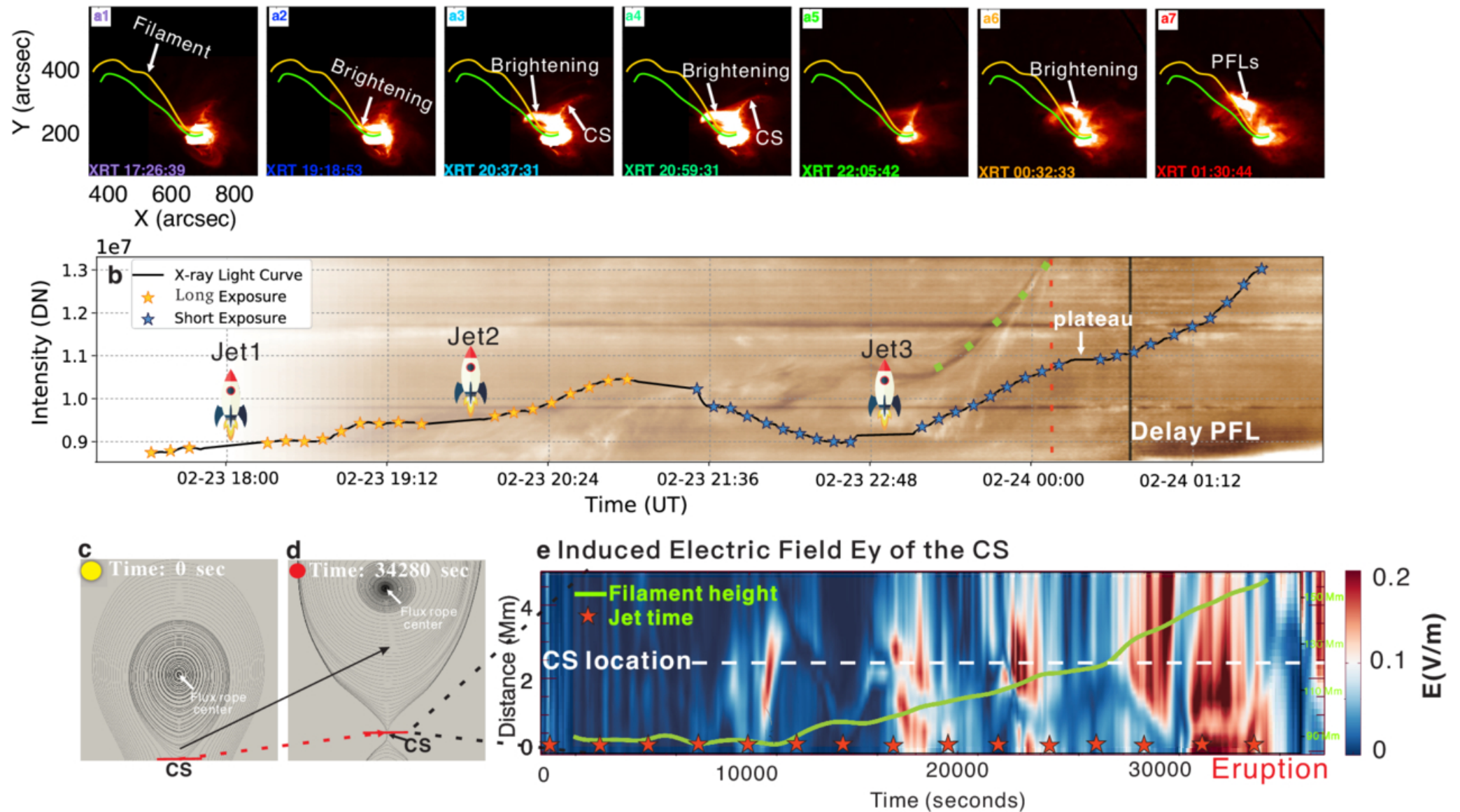
Figure 6. from Chengrui Zhou et al 2026 Astrophys. J. Lett. 1006 doi:10.3847/2041-8213/ae8540 https://dx.doi.org/10.3847/2041-8213/ae8540 © 2026. The Author(s). Published by the American Astronomical Society.
