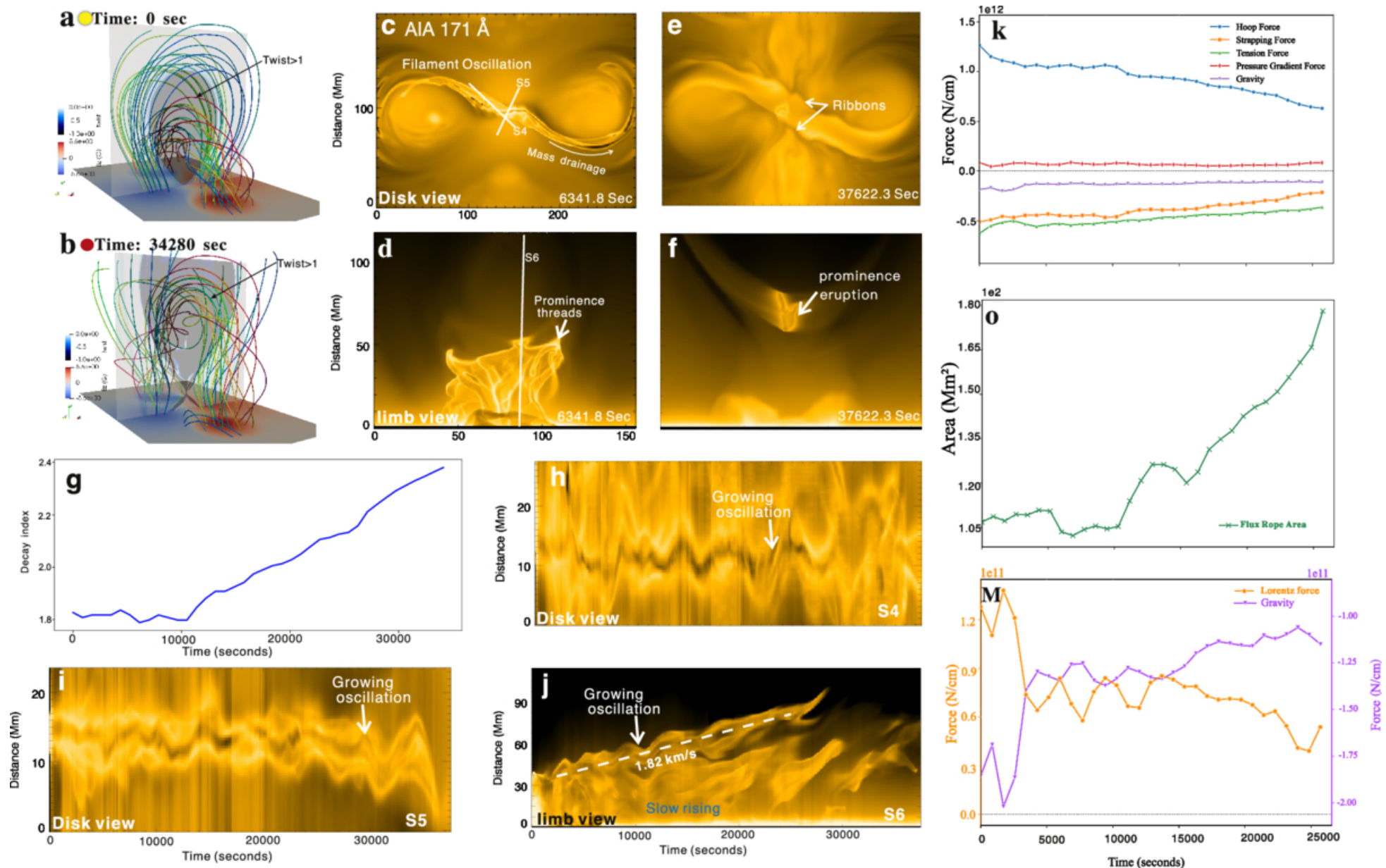
Figure 5. from Chengrui Zhou et al 2026 Astrophys. J. Lett. 1006 doi:10.3847/2041-8213/ae8540 https://dx.doi.org/10.3847/2041-8213/ae8540 © 2026. The Author(s). Published by the American Astronomical Society.
