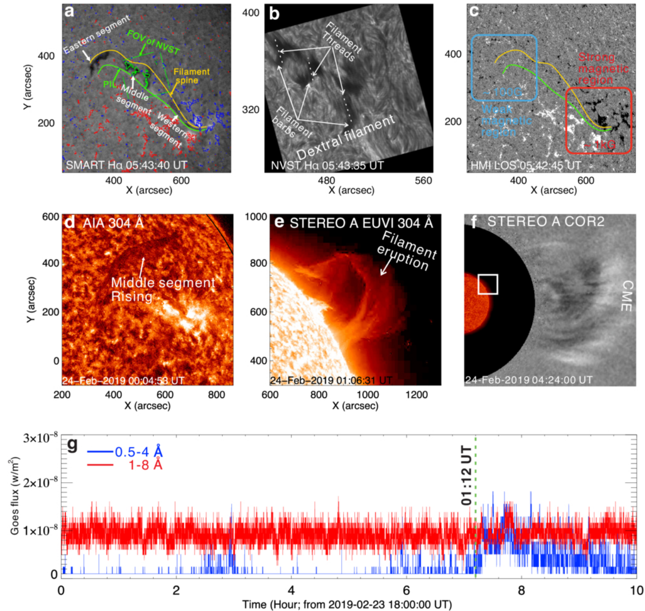
Figure 1. from Chengrui Zhou et al 2026 Astrophys. J. Lett. 1006 doi:10.3847/2041-8213/ae8540 https://dx.doi.org/10.3847/2041-8213/ae8540 © 2026. The Author(s). Published by the American Astronomical Society.
