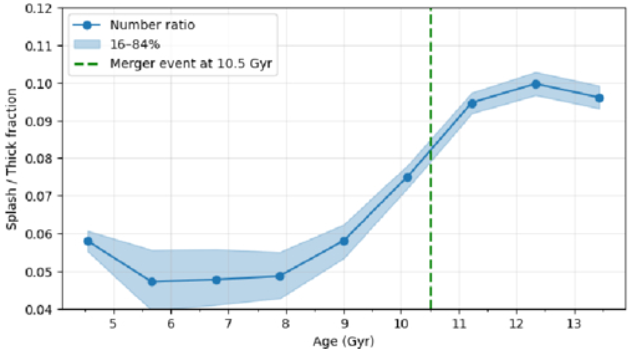
Figure A1. from Sihan Lu et al 2026 Astrophys. J. Lett. 1006 doi:10.3847/2041-8213/ae853d https://dx.doi.org/10.3847/2041-8213/ae853d © 2026. The Author(s). Published by the American Astronomical Society.
