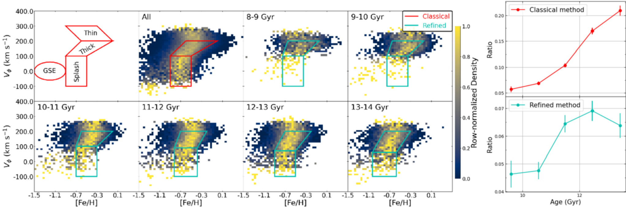
Figure 2. from Sihan Lu et al 2026 Astrophys. J. Lett. 1006 doi:10.3847/2041-8213/ae853d https://dx.doi.org/10.3847/2041-8213/ae853d © 2026. The Author(s). Published by the American Astronomical Society.
