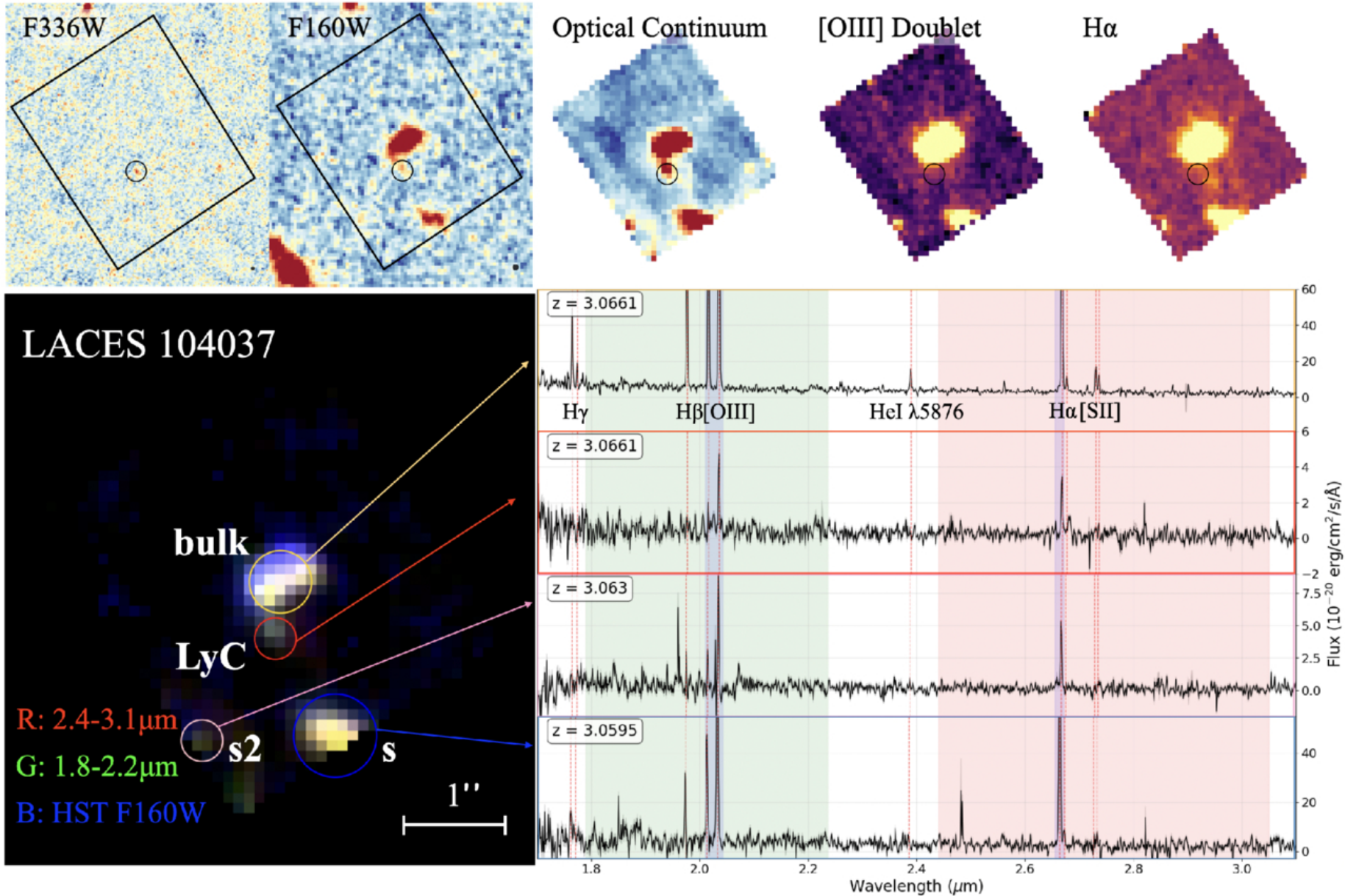
Figure 1. from Shengzhe Wang et al 2026 Astrophys. J. Lett. 1006 doi:10.3847/2041-8213/ae8523 https://dx.doi.org/10.3847/2041-8213/ae8523 © 2026. The Author(s). Published by the American Astronomical Society.
