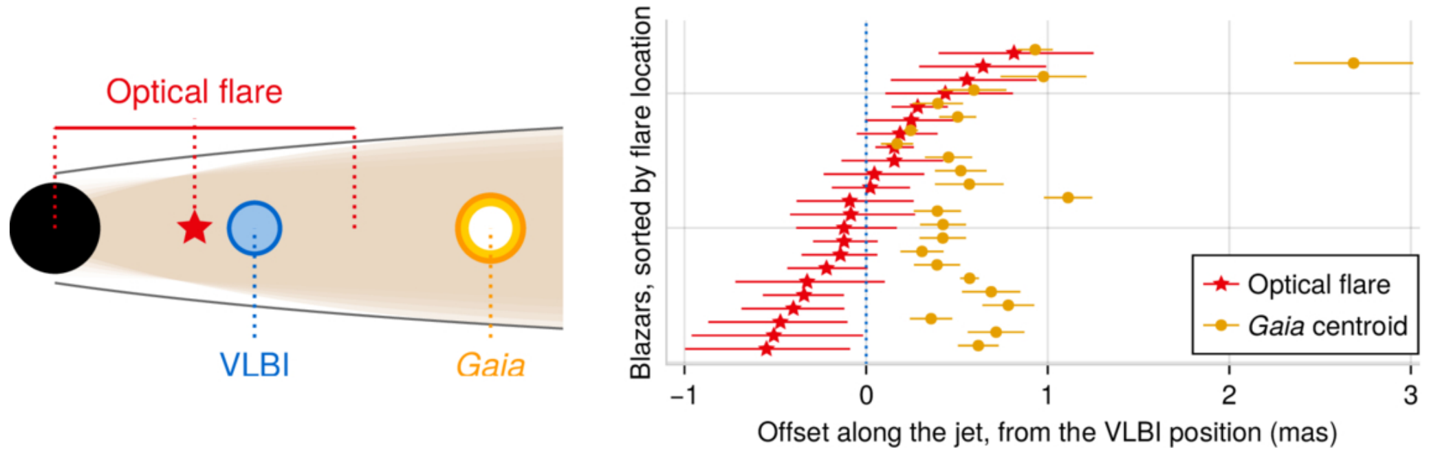
Figure 5. from A. V. Plavin 2026 Astrophys. J. Lett. 1006 doi:10.3847/2041-8213/ae84d1 https://dx.doi.org/10.3847/2041-8213/ae84d1 © 2026. The Author(s). Published by the American Astronomical Society.
