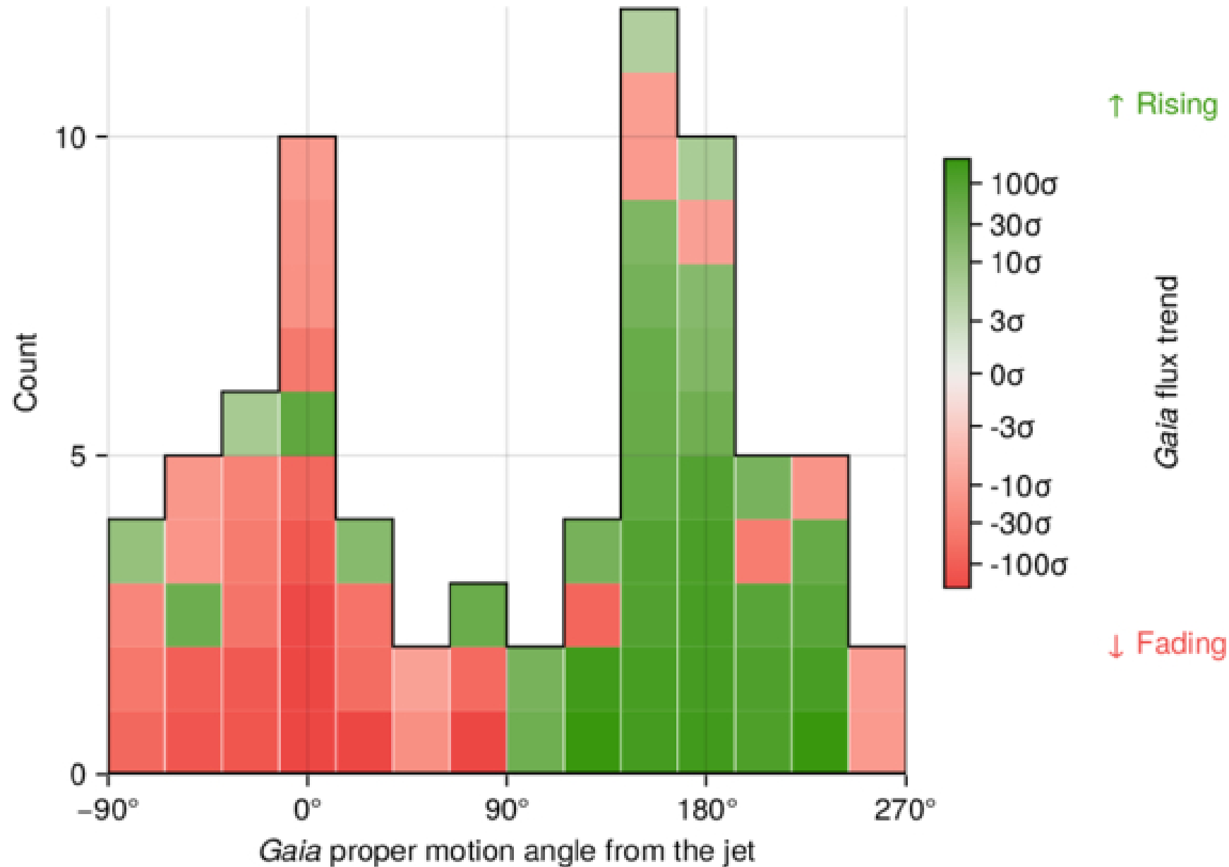
Figure 4. from A. V. Plavin 2026 Astrophys. J. Lett. 1006 doi:10.3847/2041-8213/ae84d1 https://dx.doi.org/10.3847/2041-8213/ae84d1 © 2026. The Author(s). Published by the American Astronomical Society.
