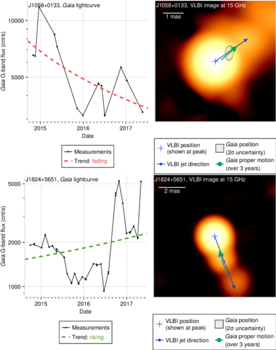
Figure 3. from A. V. Plavin 2026 Astrophys. J. Lett. 1006 doi:10.3847/2041-8213/ae84d1 https://dx.doi.org/10.3847/2041-8213/ae84d1 © 2026. The Author(s). Published by the American Astronomical Society.
