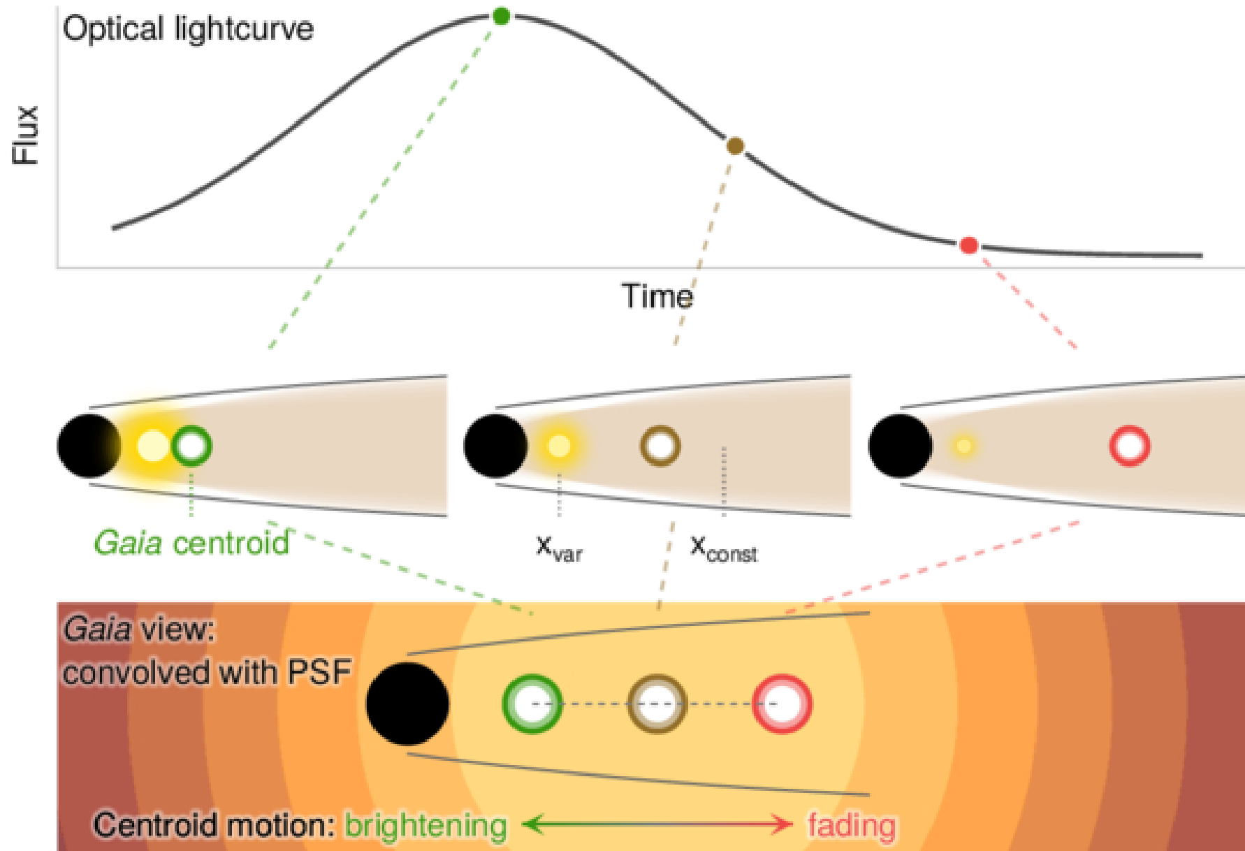
Figure 2. from A. V. Plavin 2026 Astrophys. J. Lett. 1006 doi:10.3847/2041-8213/ae84d1 https://dx.doi.org/10.3847/2041-8213/ae84d1 © 2026. The Author(s). Published by the American Astronomical Society.
