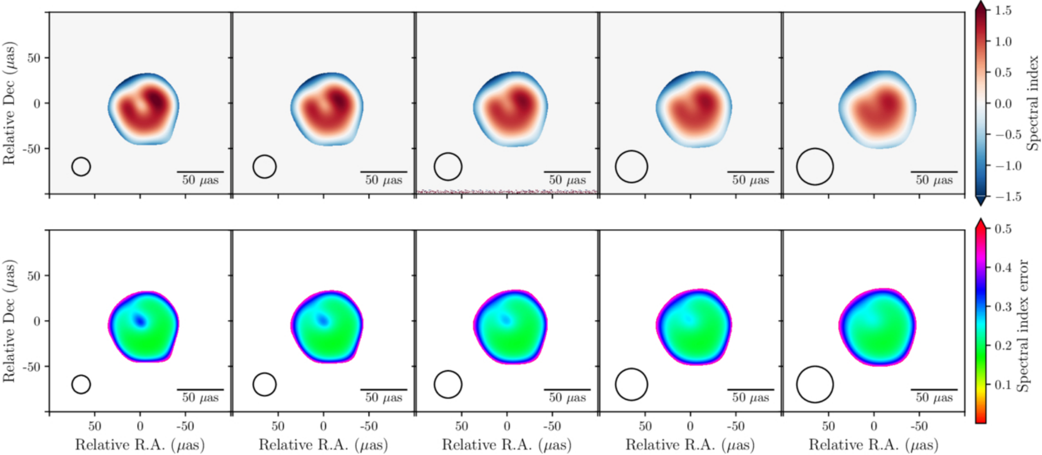
Figure 4. from Shan-Shan Zhao et al 2026 Astrophys. J. Lett. 1006 doi:10.3847/2041-8213/ae84ca https://dx.doi.org/10.3847/2041-8213/ae84ca © 2026. The Author(s). Published by the American Astronomical Society.
