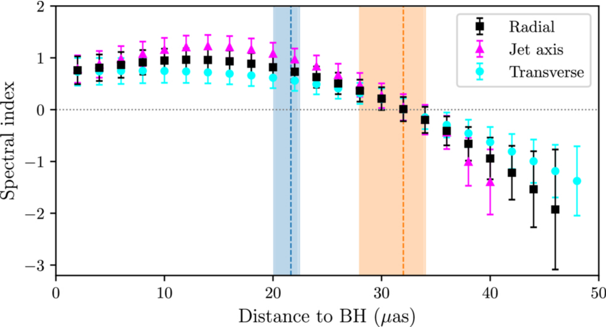
Figure 2. from Shan-Shan Zhao et al 2026 Astrophys. J. Lett. 1006 doi:10.3847/2041-8213/ae84ca https://dx.doi.org/10.3847/2041-8213/ae84ca © 2026. The Author(s). Published by the American Astronomical Society.
