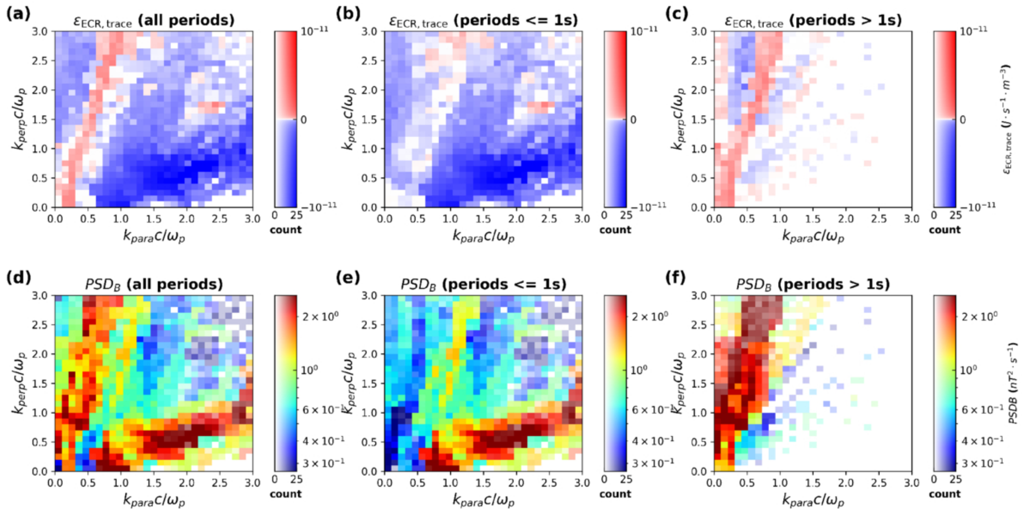
Figure 3. from Haoen Xie et al 2026 Astrophys. J. Lett. 1006 doi:10.3847/2041-8213/ae84c8 https://dx.doi.org/10.3847/2041-8213/ae84c8 © 2026. The Author(s). Published by the American Astronomical Society.
