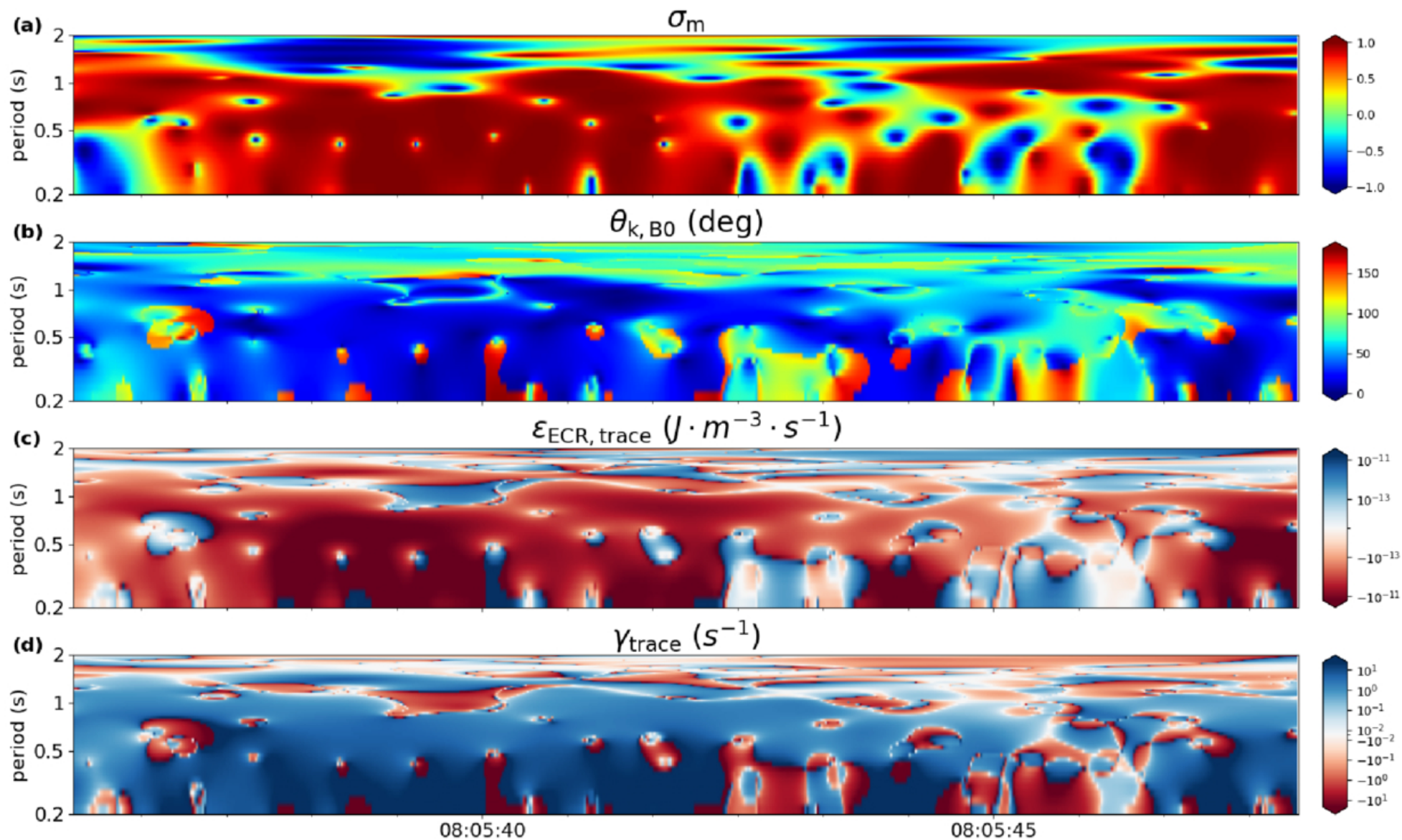
Figure 2. from Haoen Xie et al 2026 Astrophys. J. Lett. 1006 doi:10.3847/2041-8213/ae84c8 https://dx.doi.org/10.3847/2041-8213/ae84c8 © 2026. The Author(s). Published by the American Astronomical Society.
