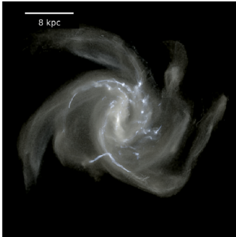
Figure 3. from Leindert A. Boogaard et al 2026 Astrophys. J. Lett. 1006 doi:10.3847/2041-8213/ae84c7 https://dx.doi.org/10.3847/2041-8213/ae84c7 © 2026. The Author(s). Published by the American Astronomical Society.
