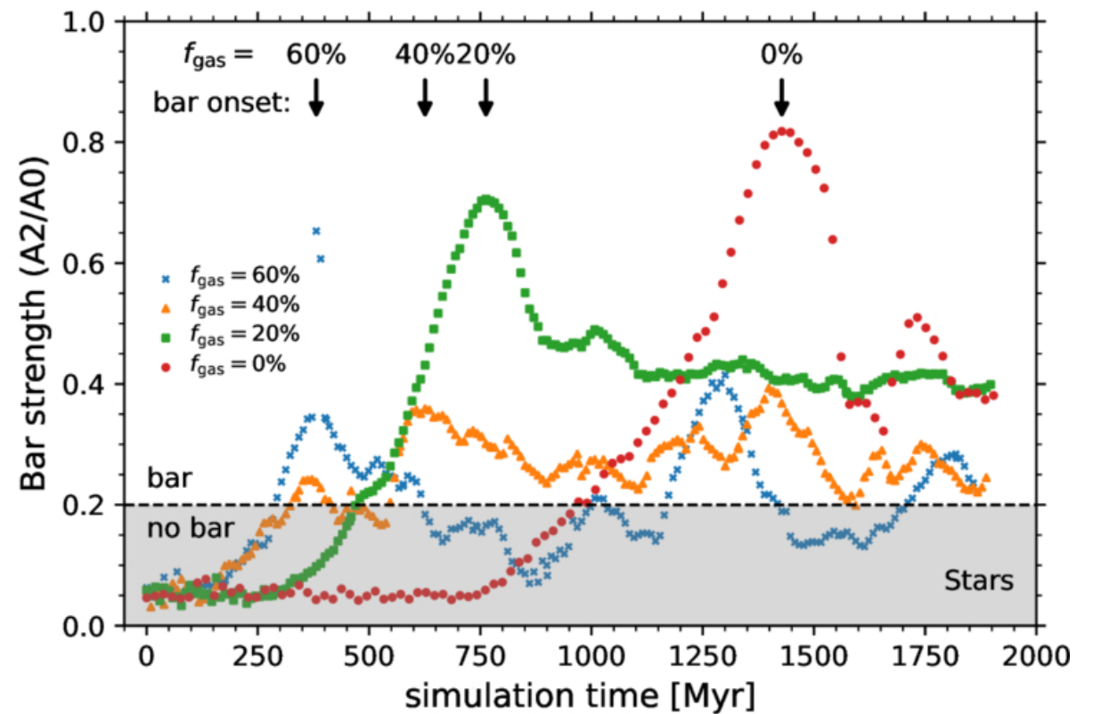
Figure 3. from Leindert A. Boogaard et al 2026 Astrophys. J. Lett. 1006 doi:10.3847/2041-8213/ae84c7 https://dx.doi.org/10.3847/2041-8213/ae84c7 © 2026. The Author(s). Published by the American Astronomical Society.
