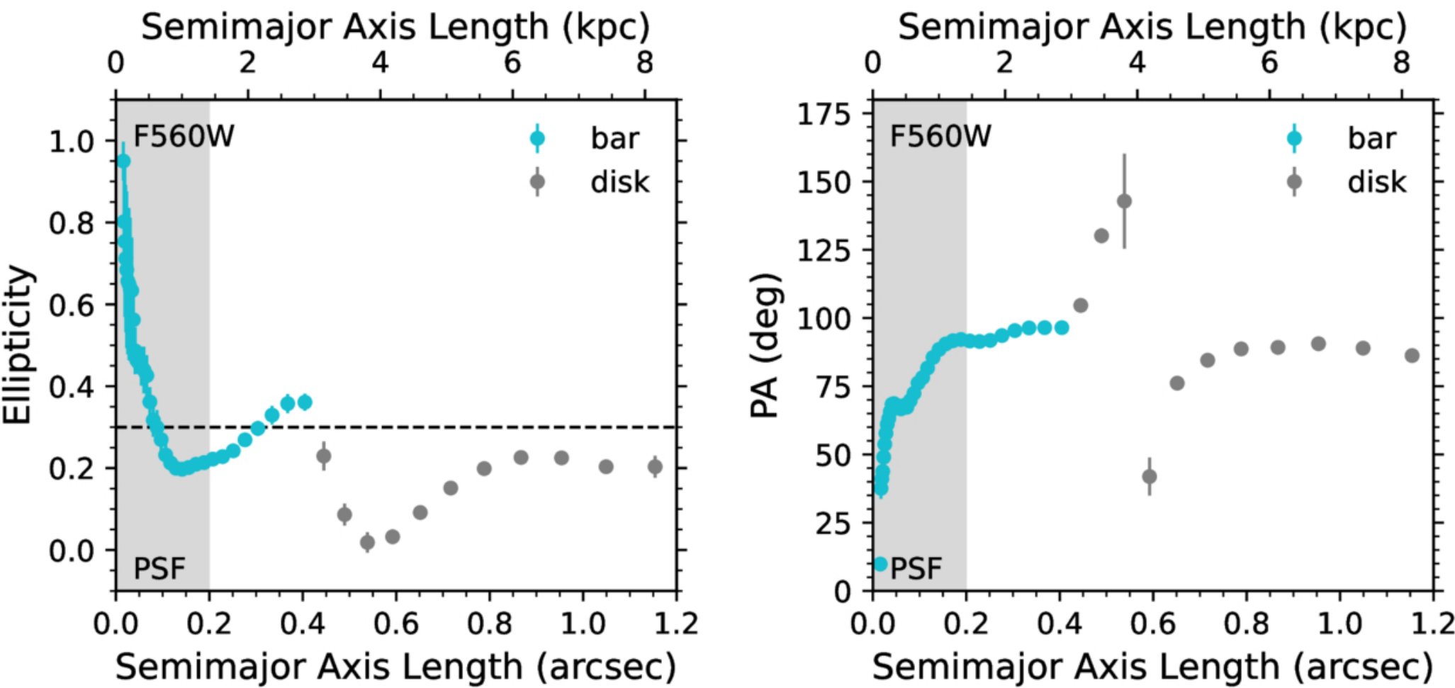
Figure 2. from Leindert A. Boogaard et al 2026 Astrophys. J. Lett. 1006 doi:10.3847/2041-8213/ae84c7 https://dx.doi.org/10.3847/2041-8213/ae84c7 © 2026. The Author(s). Published by the American Astronomical Society.
