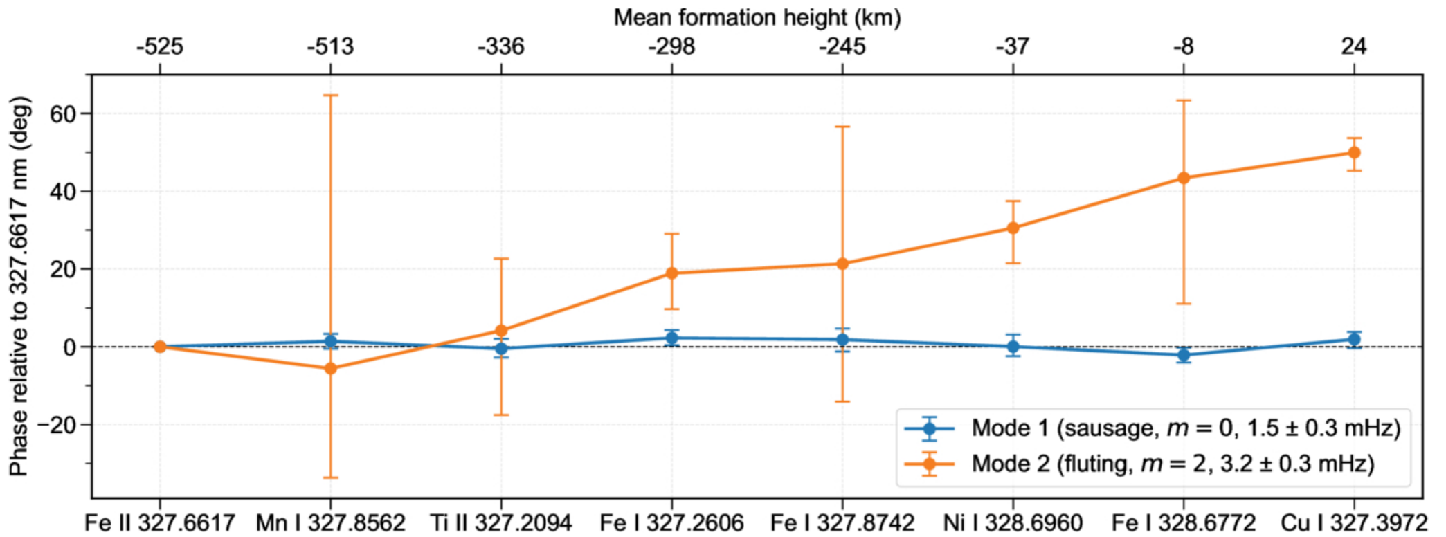
Figure 3. from Shahin Jafarzadeh et al 2026 Astrophys. J. Lett. 1005 doi:10.3847/2041-8213/ae84bf https://dx.doi.org/10.3847/2041-8213/ae84bf © 2026. The Author(s). Published by the American Astronomical Society.
