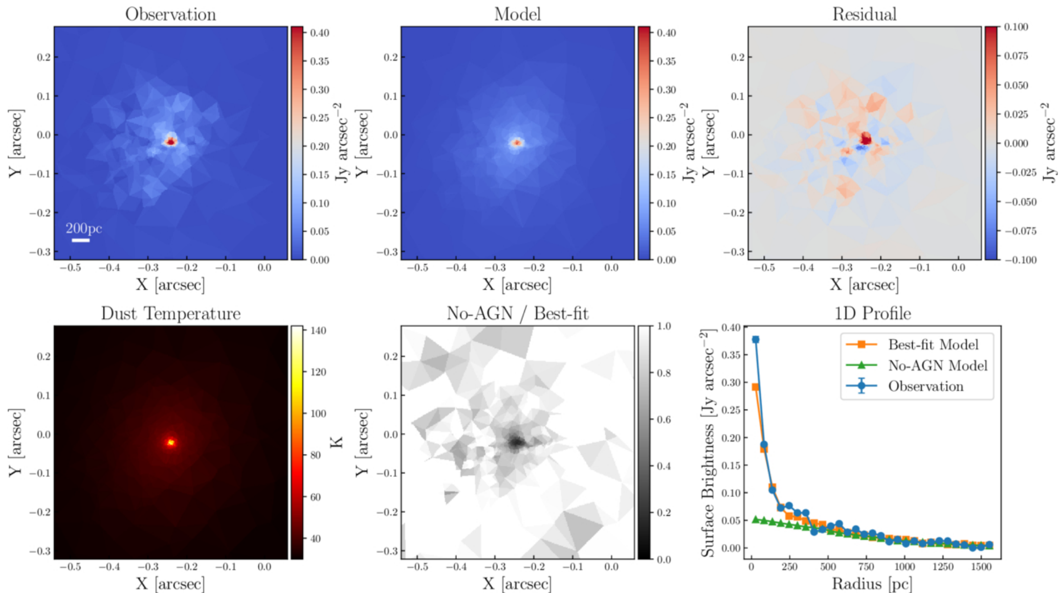
Figure 4. from Minghao Yue et al 2026 Astrophys. J. Lett. 1006 doi:10.3847/2041-8213/ae84bc https://dx.doi.org/10.3847/2041-8213/ae84bc © 2026. The Author(s). Published by the American Astronomical Society.
