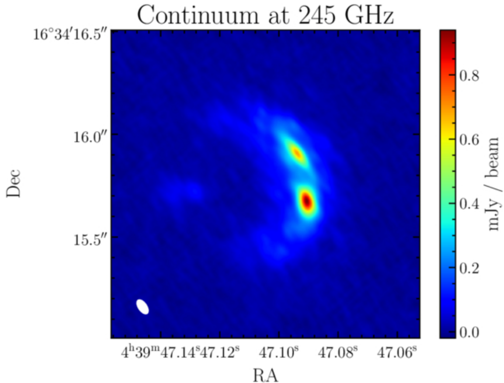
Figure 1. from Minghao Yue et al 2026 Astrophys. J. Lett. 1006 doi:10.3847/2041-8213/ae84bc https://dx.doi.org/10.3847/2041-8213/ae84bc © 2026. The Author(s). Published by the American Astronomical Society.
