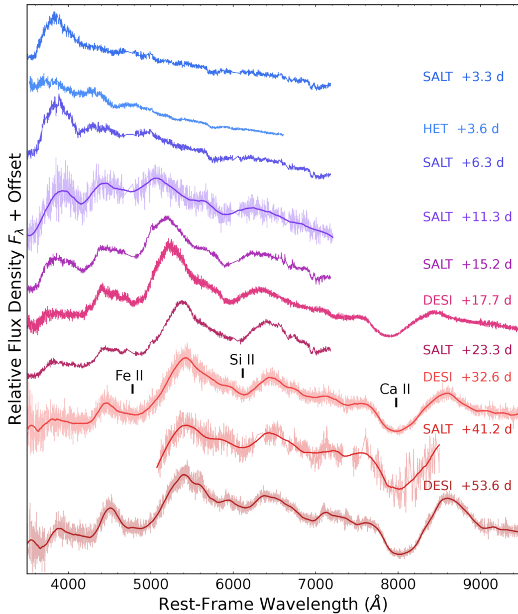
Figure 6. from Brendan O'Connor et al 2026 Astrophys. J. Lett. 1006 doi:10.3847/2041-8213/ae84ba https://dx.doi.org/10.3847/2041-8213/ae84ba © 2026. The Author(s). Published by the American Astronomical Society.
