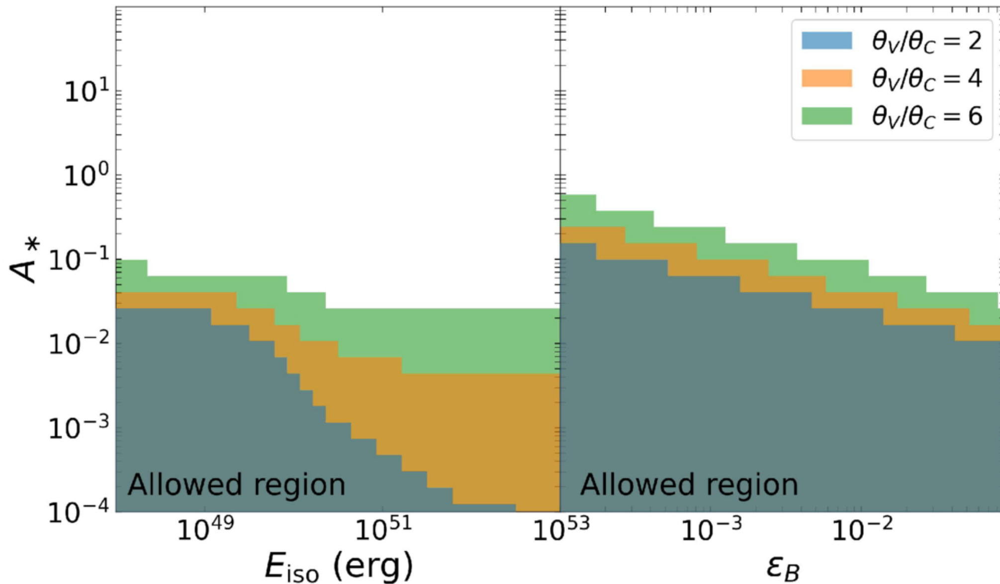
Figure 18. from Brendan O'Connor et al 2026 Astrophys. J. Lett. 1006 doi:10.3847/2041-8213/ae84ba https://dx.doi.org/10.3847/2041-8213/ae84ba © 2026. The Author(s). Published by the American Astronomical Society.
