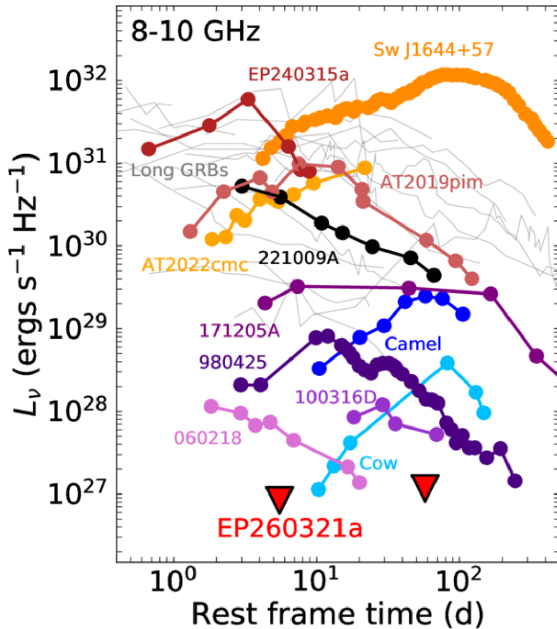
Figure 16. from Brendan O'Connor et al 2026 Astrophys. J. Lett. 1006 doi:10.3847/2041-8213/ae84ba https://dx.doi.org/10.3847/2041-8213/ae84ba © 2026. The Author(s). Published by the American Astronomical Society.
