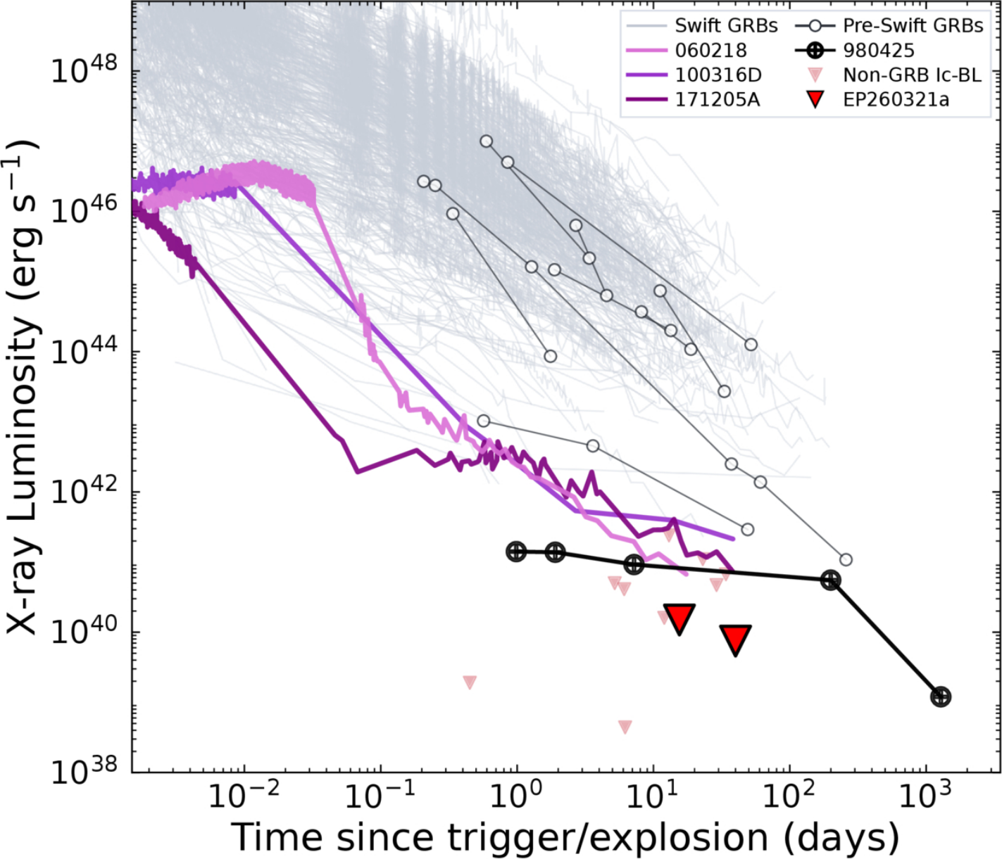
Figure 15. from Brendan O'Connor et al 2026 Astrophys. J. Lett. 1006 doi:10.3847/2041-8213/ae84ba https://dx.doi.org/10.3847/2041-8213/ae84ba © 2026. The Author(s). Published by the American Astronomical Society.
