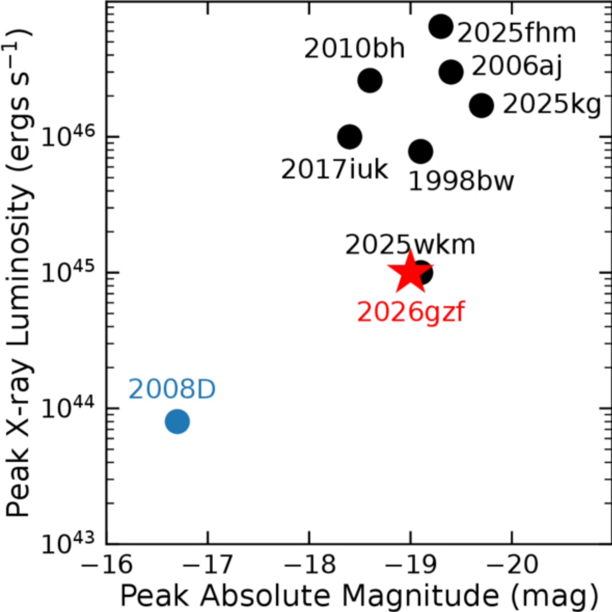
Figure 13. from Brendan O'Connor et al 2026 Astrophys. J. Lett. 1006 doi:10.3847/2041-8213/ae84ba https://dx.doi.org/10.3847/2041-8213/ae84ba © 2026. The Author(s). Published by the American Astronomical Society.
