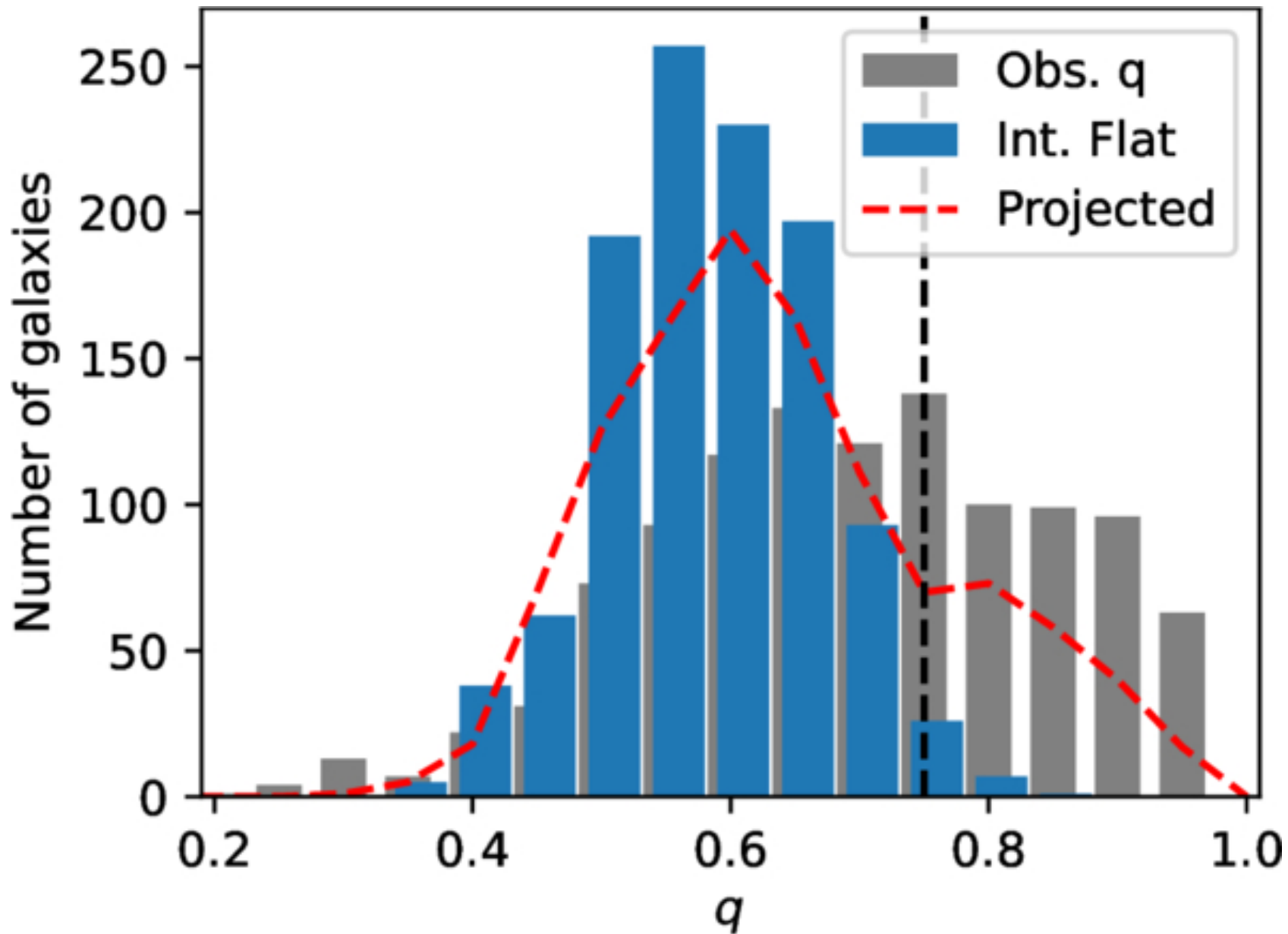
Figure 9. from Sanjaya Paudel et al 2026 Astrophys. J. Lett. 1006 doi:10.3847/2041-8213/ae8442 https://dx.doi.org/10.3847/2041-8213/ae8442 © 2026. The Author(s). Published by the American Astronomical Society.
