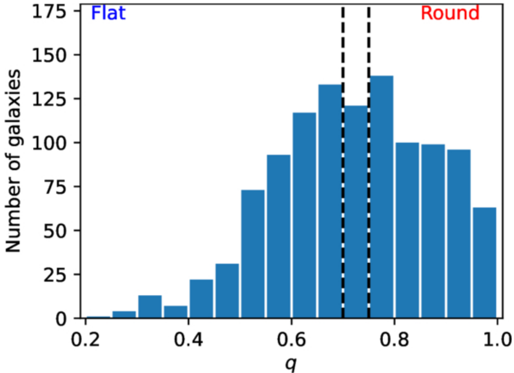
Figure 2. from Sanjaya Paudel et al 2026 Astrophys. J. Lett. 1006 doi:10.3847/2041-8213/ae8442 https://dx.doi.org/10.3847/2041-8213/ae8442 © 2026. The Author(s). Published by the American Astronomical Society.
