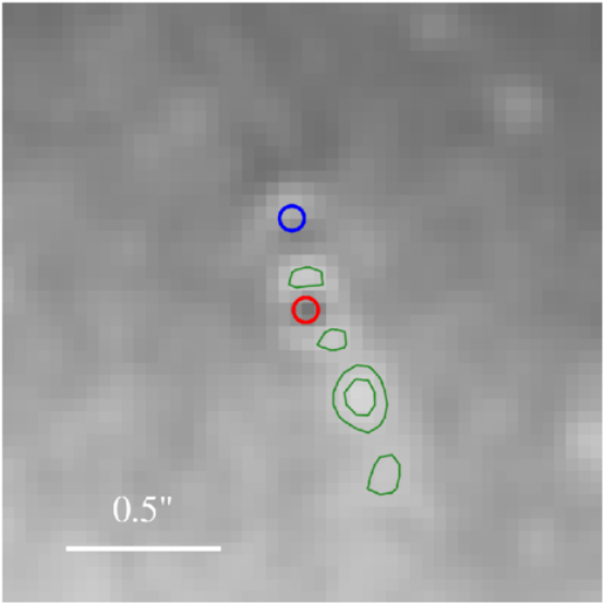
Residual stack (F277W–F444W)
