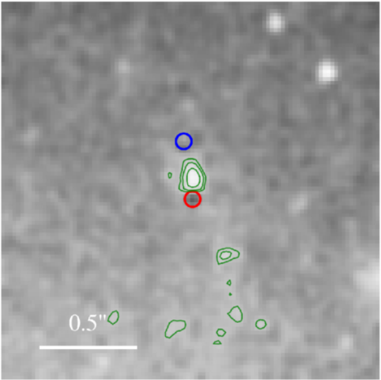
Residual stack (F090W–F210M)
